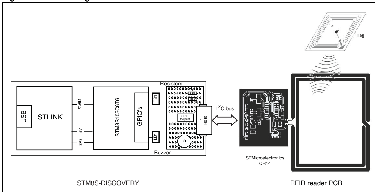
Figure 1. Short range RFID reader solution
