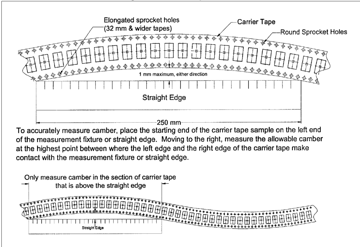
Figure 7. Camber requirements
