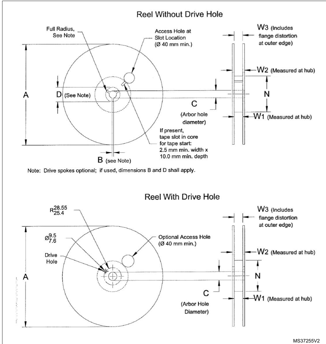
Figure 1. Reel diagram
