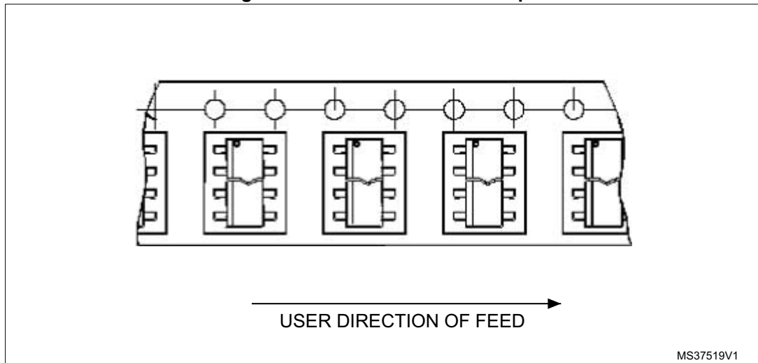
Figure 4. Device orientation on tape
