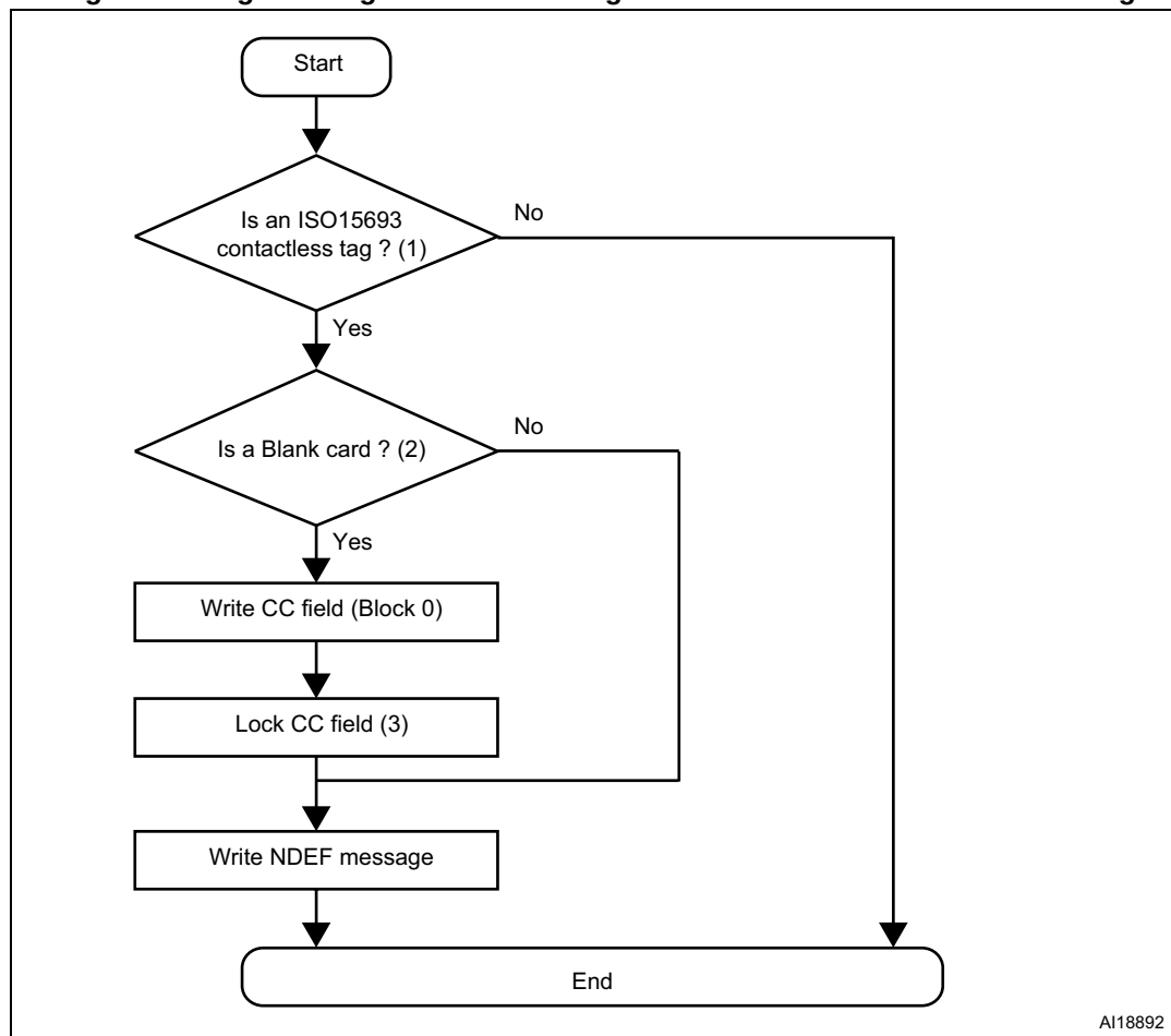
Figure 5. Programming an NDEF message in an ISO/IEC 15693 contactless tag
