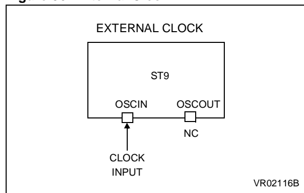
Figure 36. External Clock
