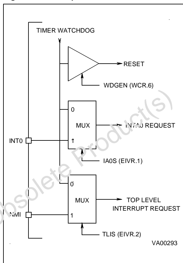
Figure 51. Interrupt Sources
