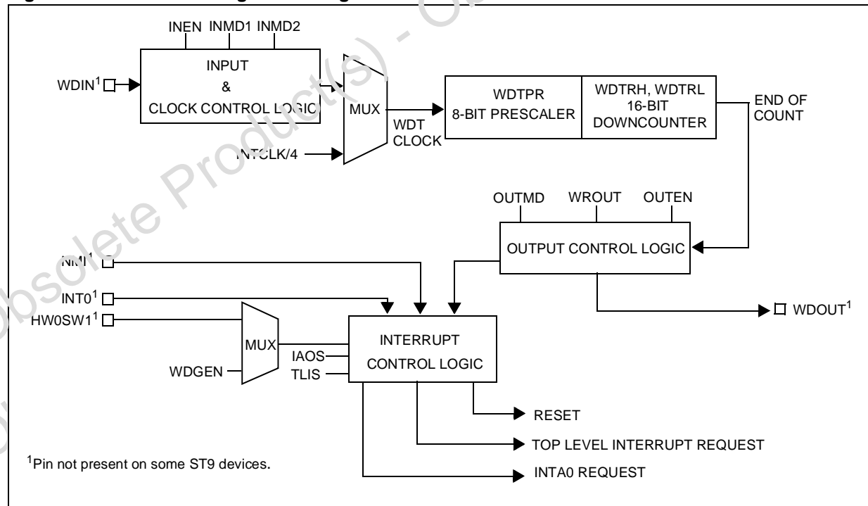
Figure 49. Timer/Watchdog Block Diagram
