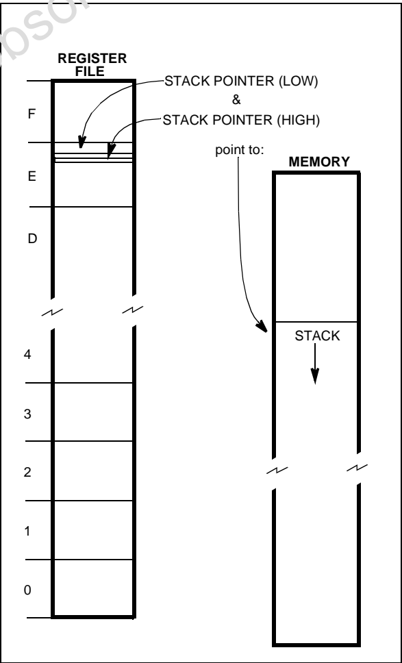
Figure 10. External Stack Mode
