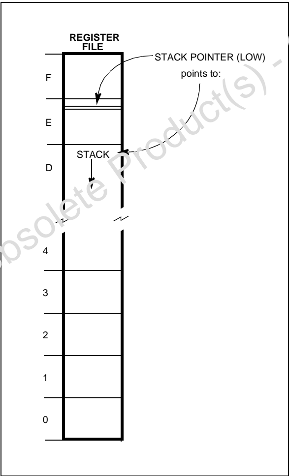
Figure 9. Internal Stack Mode
