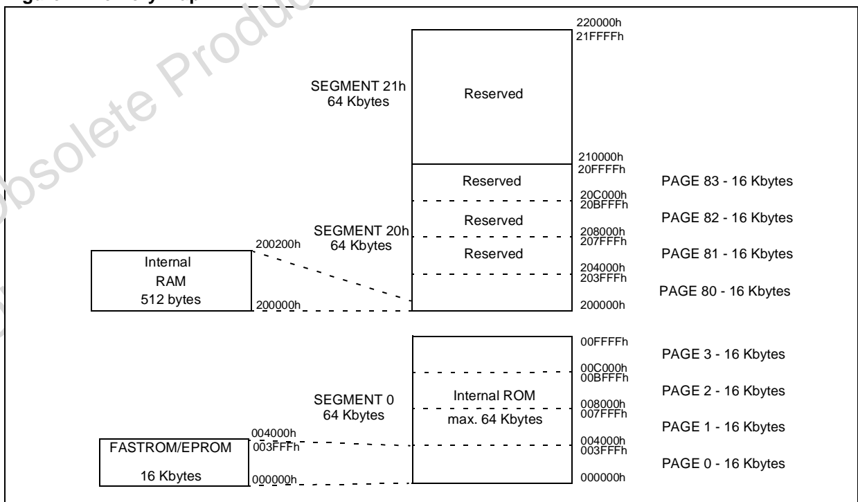
Figure 2. Memory Map
