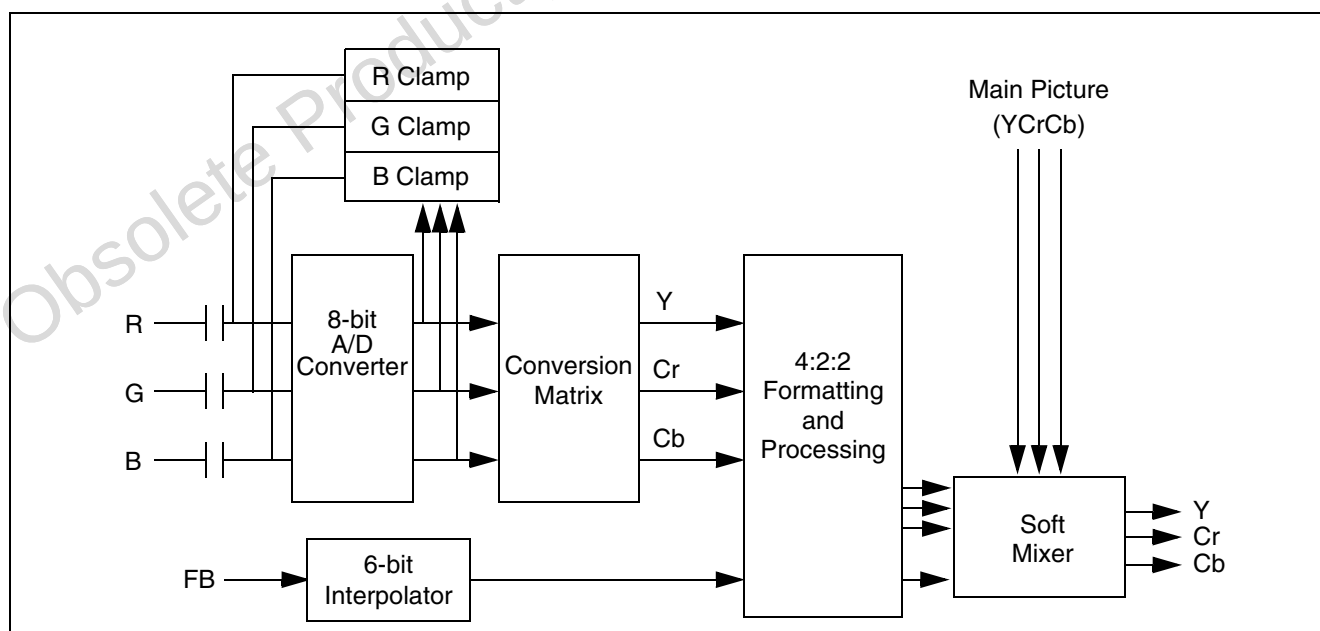
Figure 17: RGB Capture and Mixing with Main Picture
