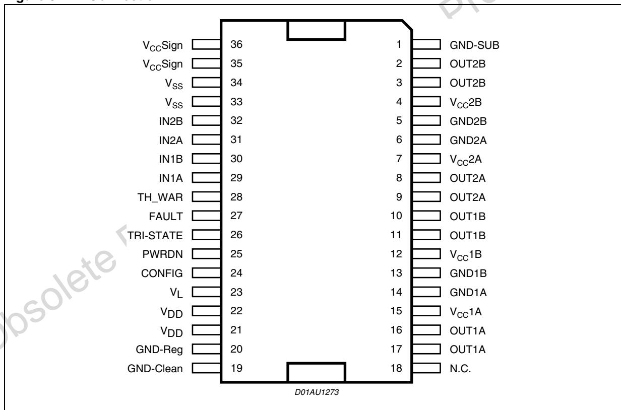
Figure 3. Pin Connection
