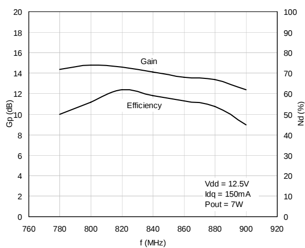
Figure 4. Gain &amp; Efficiency Vs Frequency
