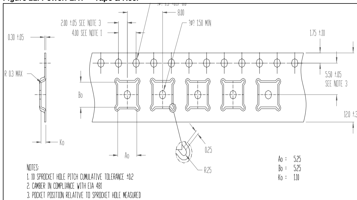
Figure 11. PowerFLAT™ Tape &amp; Reel
