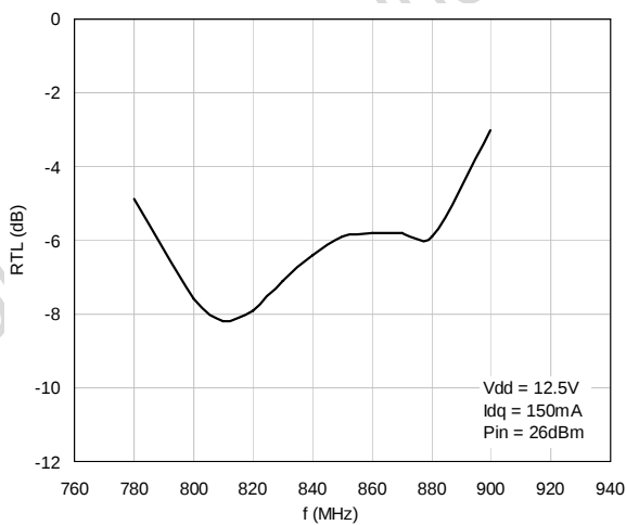
Figure 7. Input Return Loss Vs Frequency
