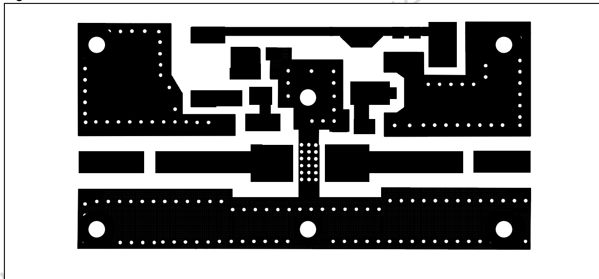
Figure 9. Photomaster
