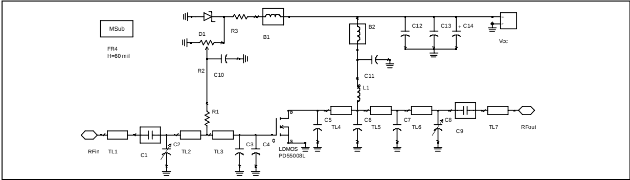
Figure 8. Test Circuit
