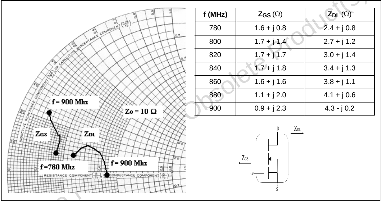
Figure 2. Impedance data
