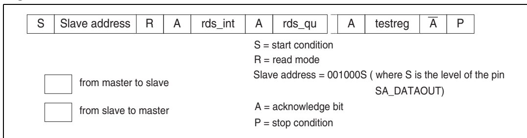
Figure 15. I 2 C read transfer
