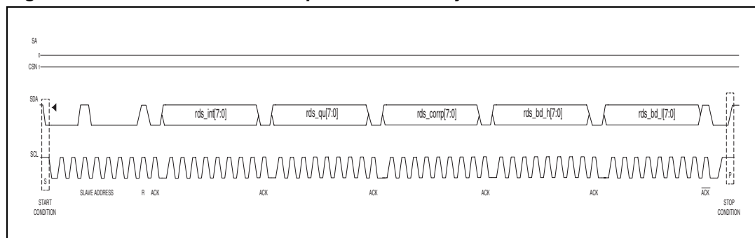
Figure 16. I 2 C read access example 1: read of 5 bytes
