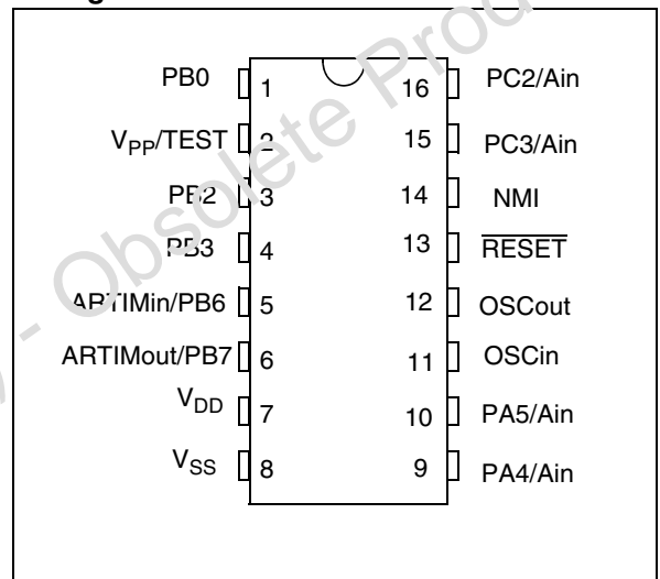
Figure 2. ST62T52C, E62C and TC2C Pin Configuration
