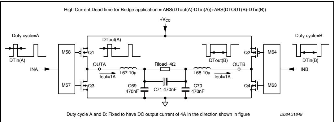
Figure 4. Test circuit 2
