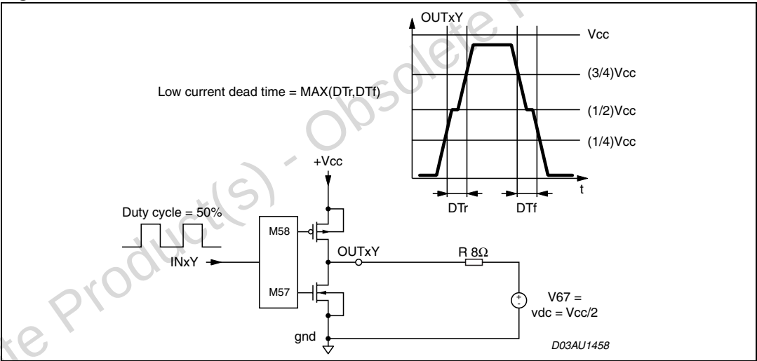
Figure 3. Test circuit 1
