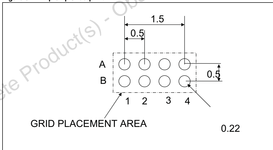
Figure 6. Flip-chip 8 footprint
