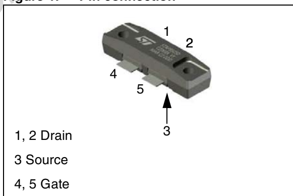
Figure 1. Pin connection
