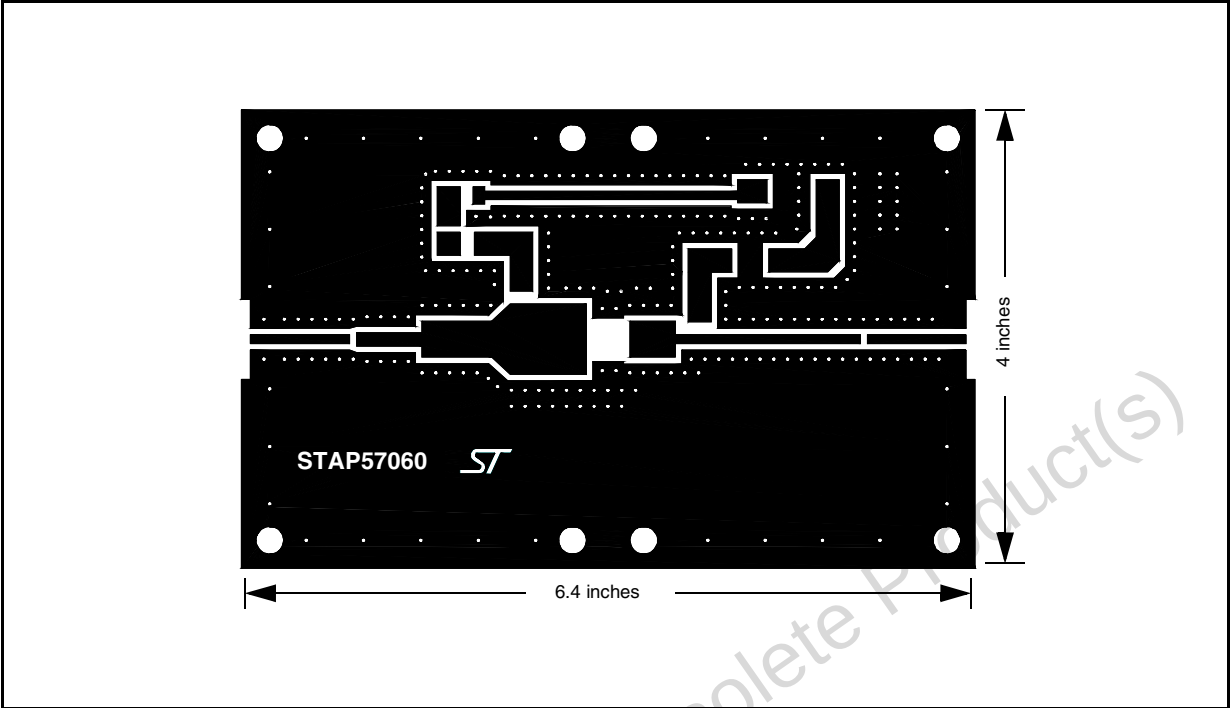
Figure 16. Test circuit photomaster
