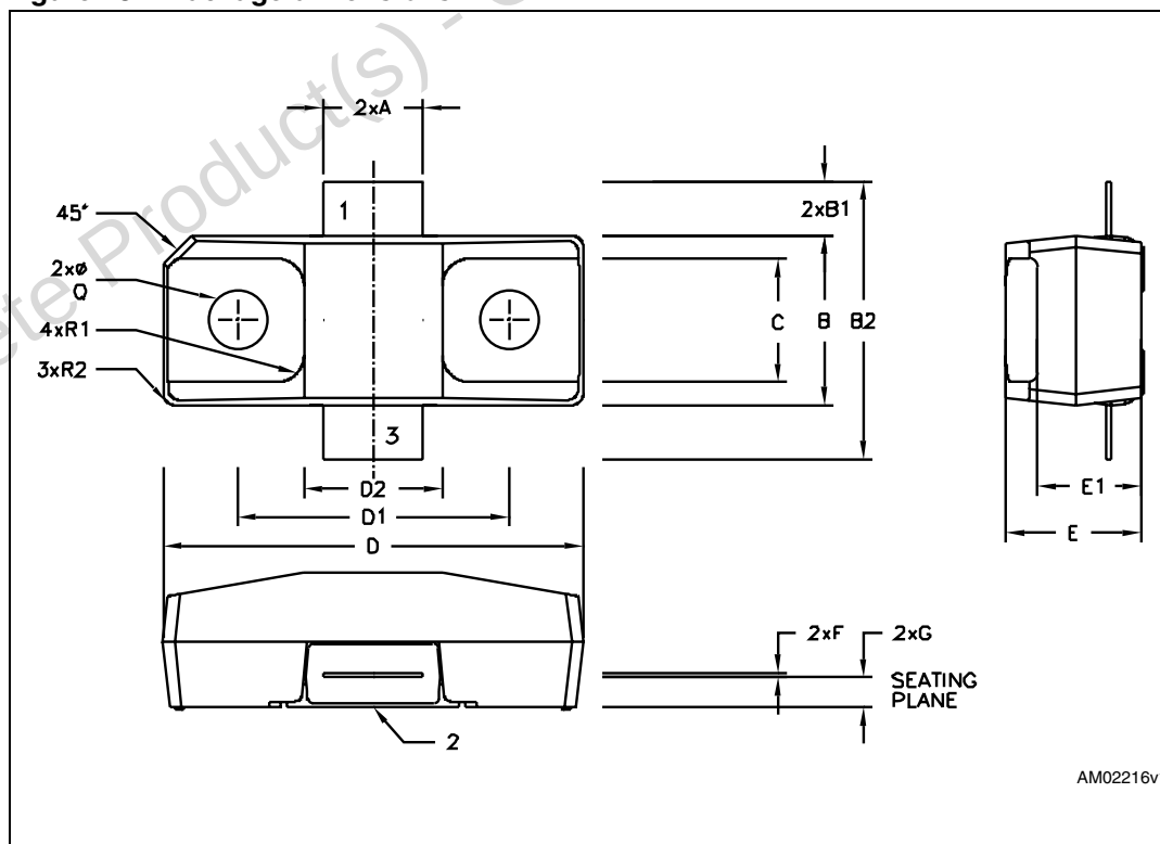
Figure 18. Package dimensions
