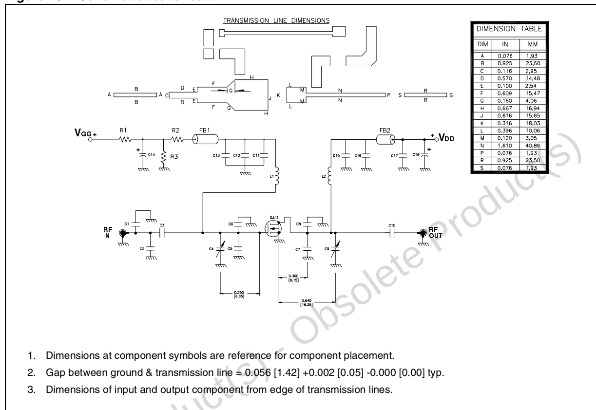
Figure 15. Schematic test circuit
