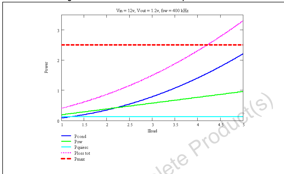
Figure 20. Estimation of the internal power losses
