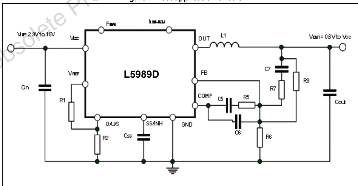
Figure 1. Test application circuit
