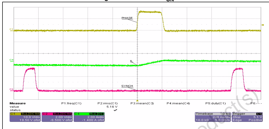
Figure 11. Minimum T_{ON}
