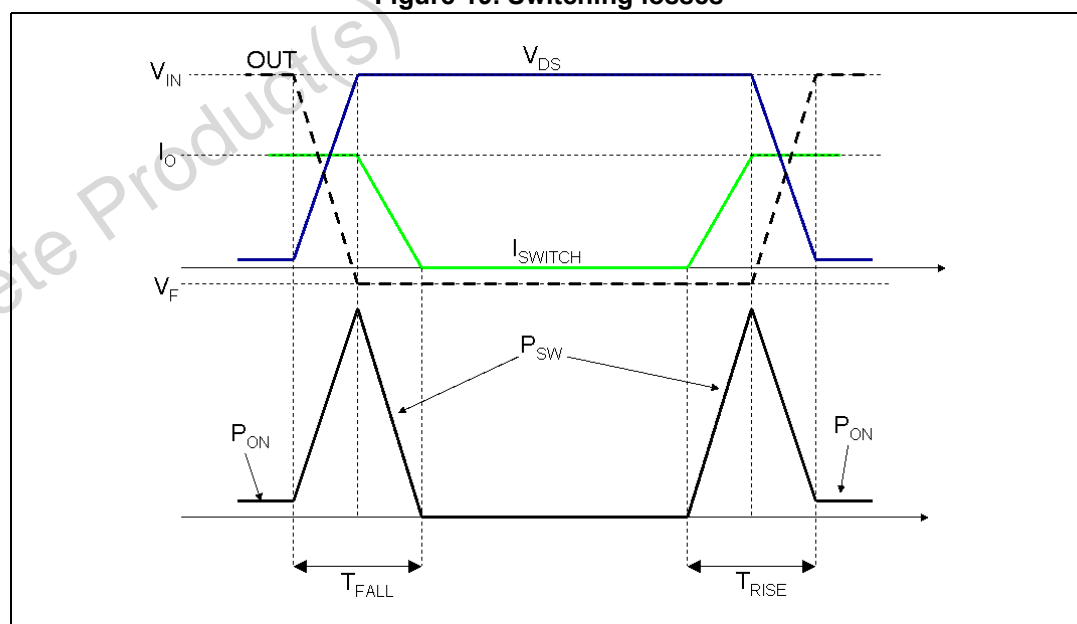
Figure 19. Switching losses
