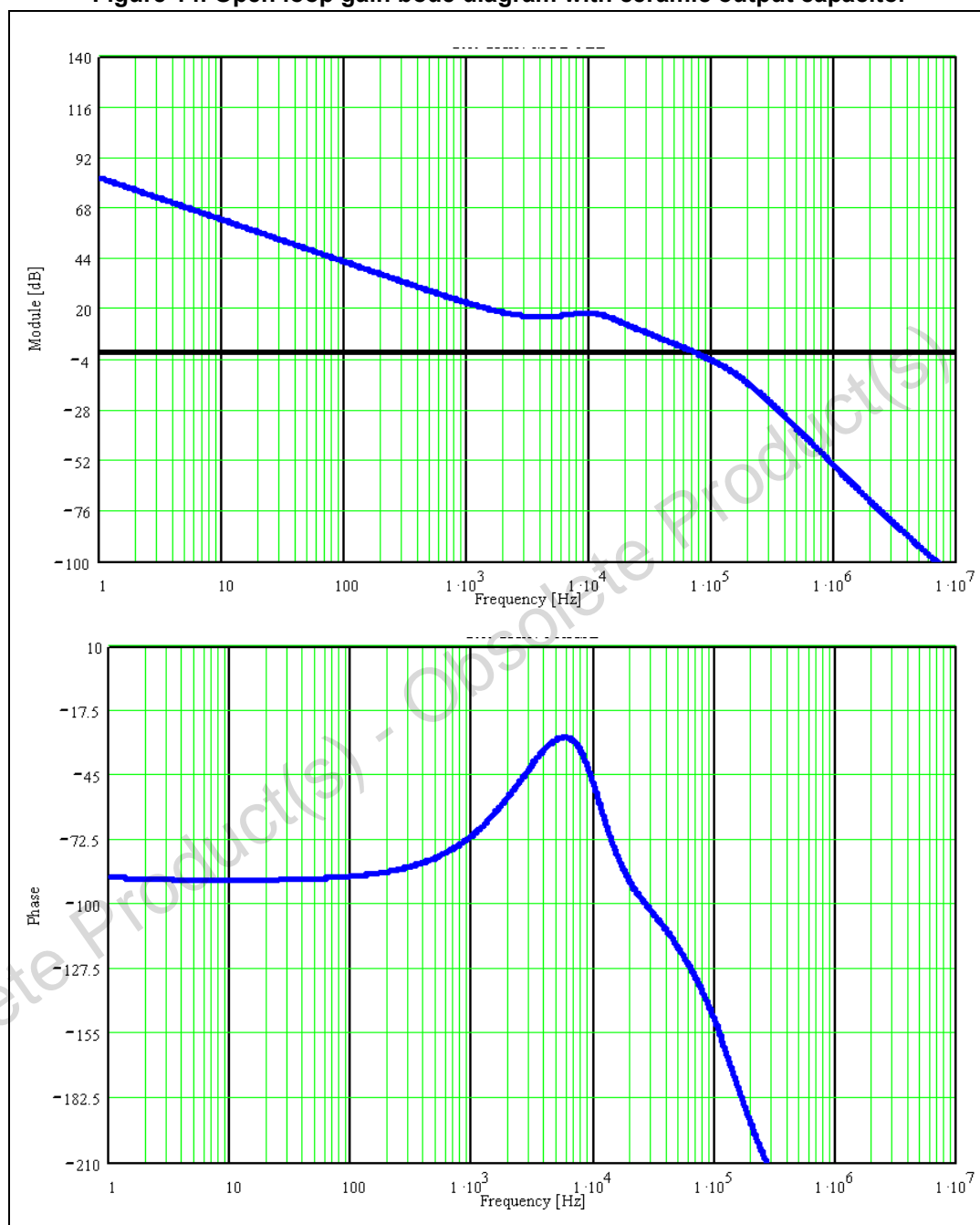
Figure 14. Open loop gain bode diagram with ceramic output capacitor
