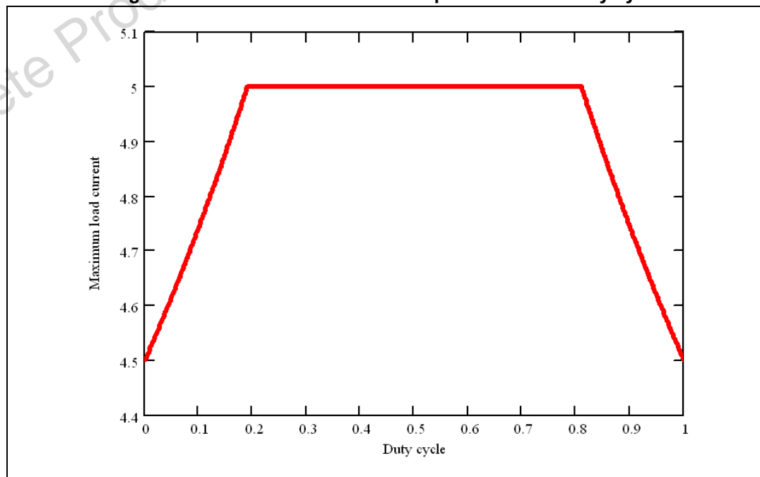
Figure 18. Maximum continuous output current vs. duty cycle
