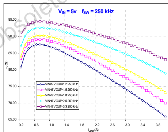
Figure 34. Efficiency vs. output current
