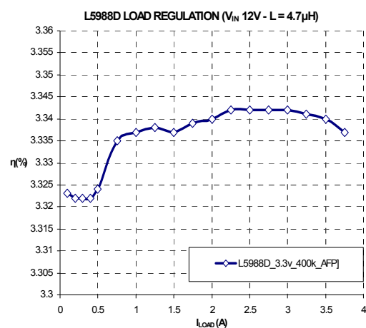
Figure 36. Load regulation
