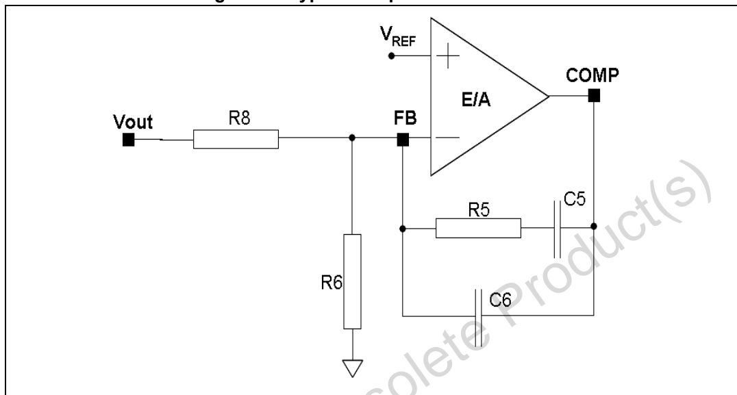
Figure 15. Type II compensation network
