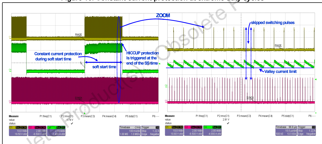
Figure 10. Constant current protection at extreme duty cycles
