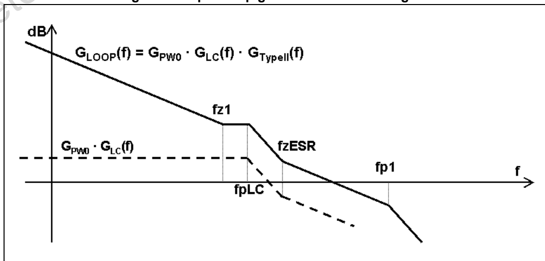
Figure 16. Open loop gain: module bode diagram
