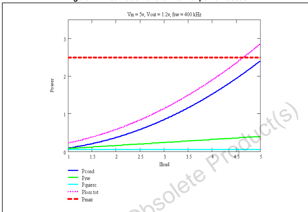
Figure 21. Estimation of the internal power losses
