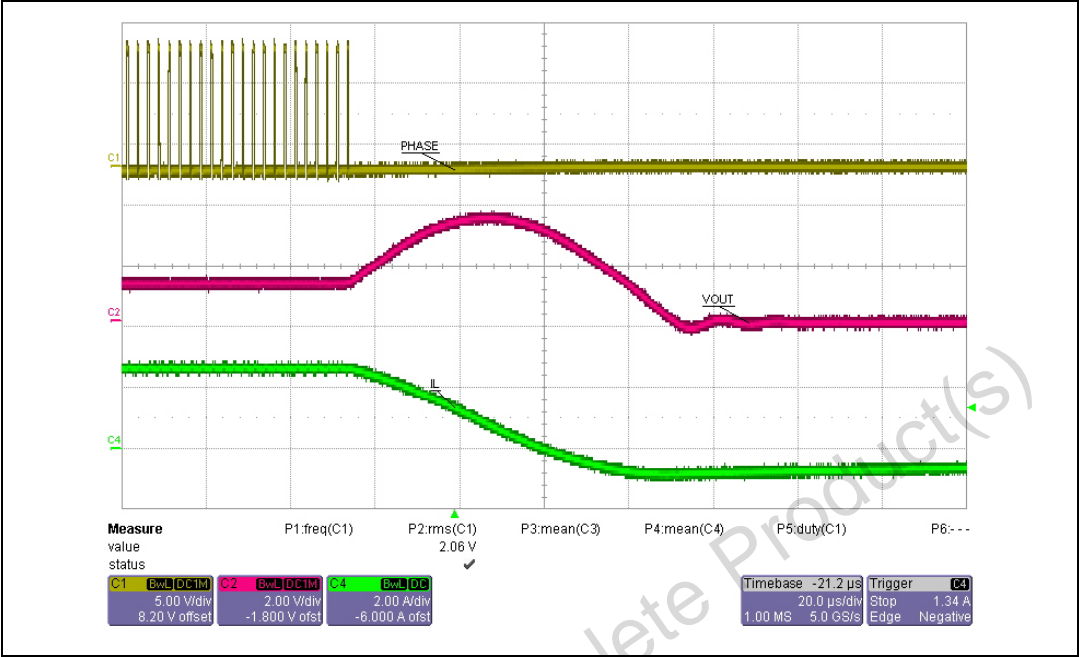
Figure 9. OVP latched
