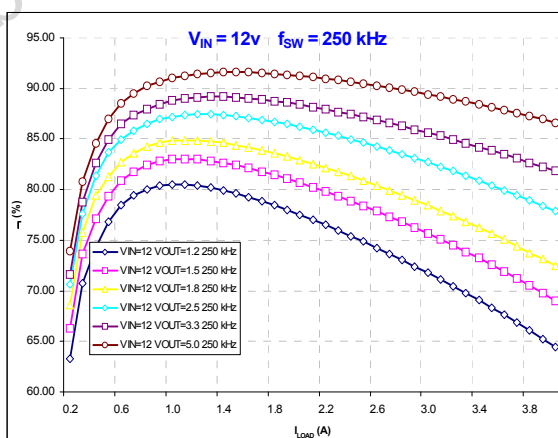
Figure 35. Efficiency vs. output current
