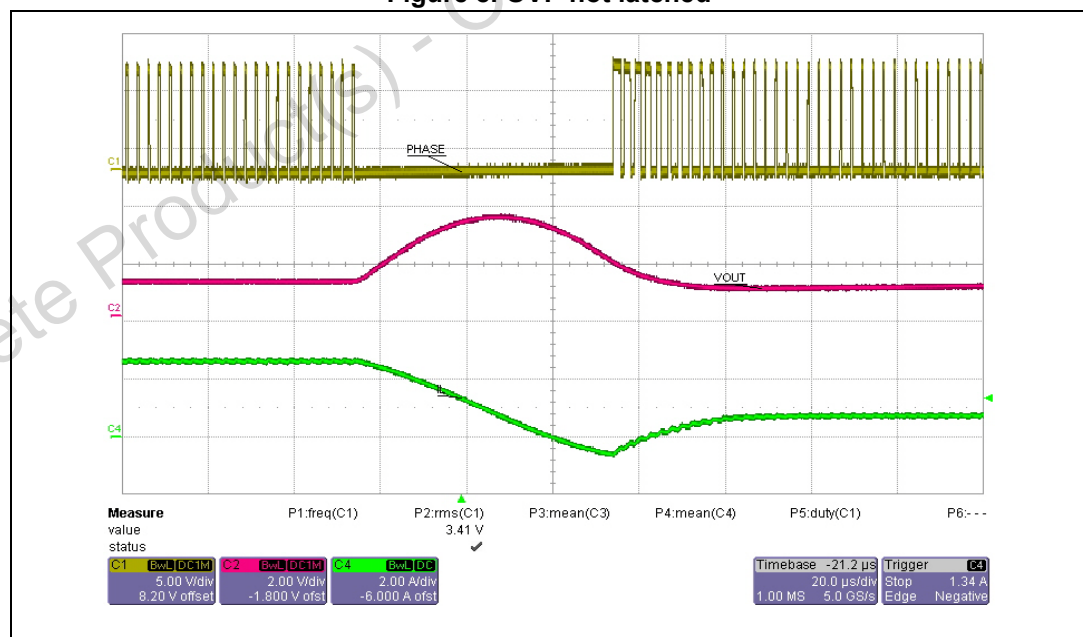
Figure 8. OVP not latched
