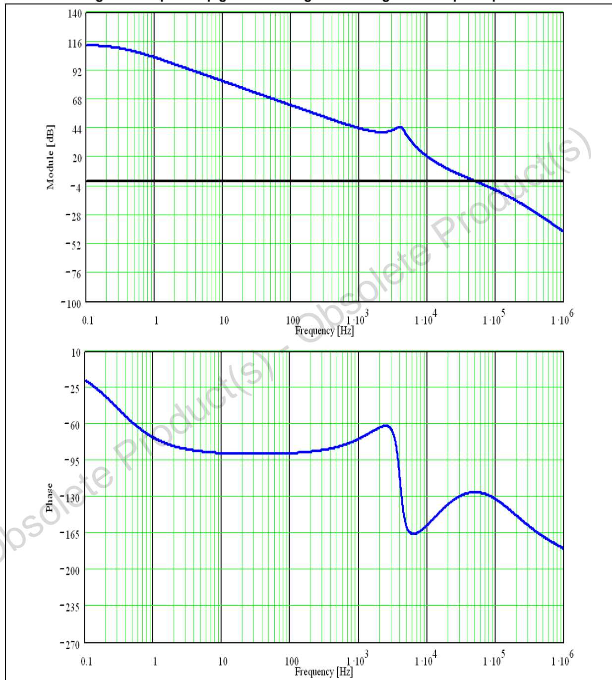
Figure 17. Open loop gain bode diagram with high ESR output capacitor
