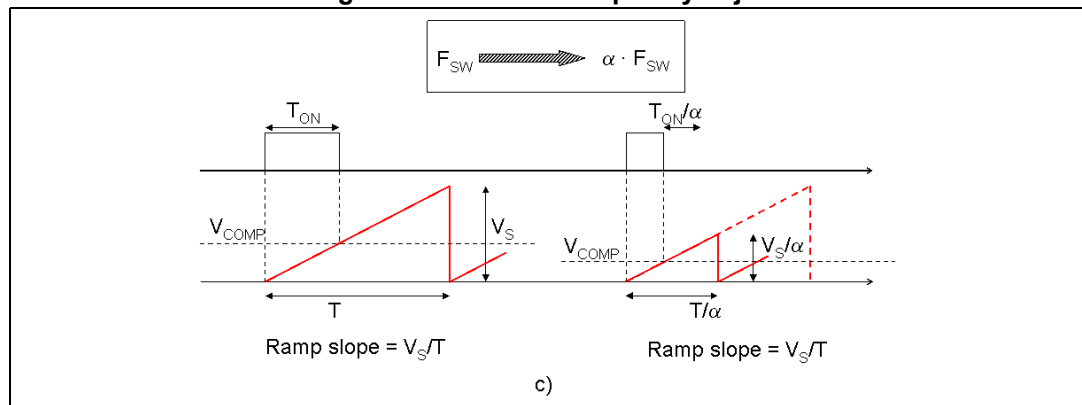
Figure 7. Sawtooth: frequency adjust
