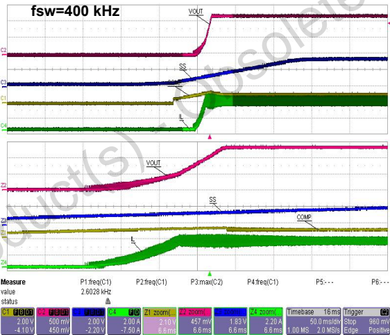
Figure 39. Soft-start
