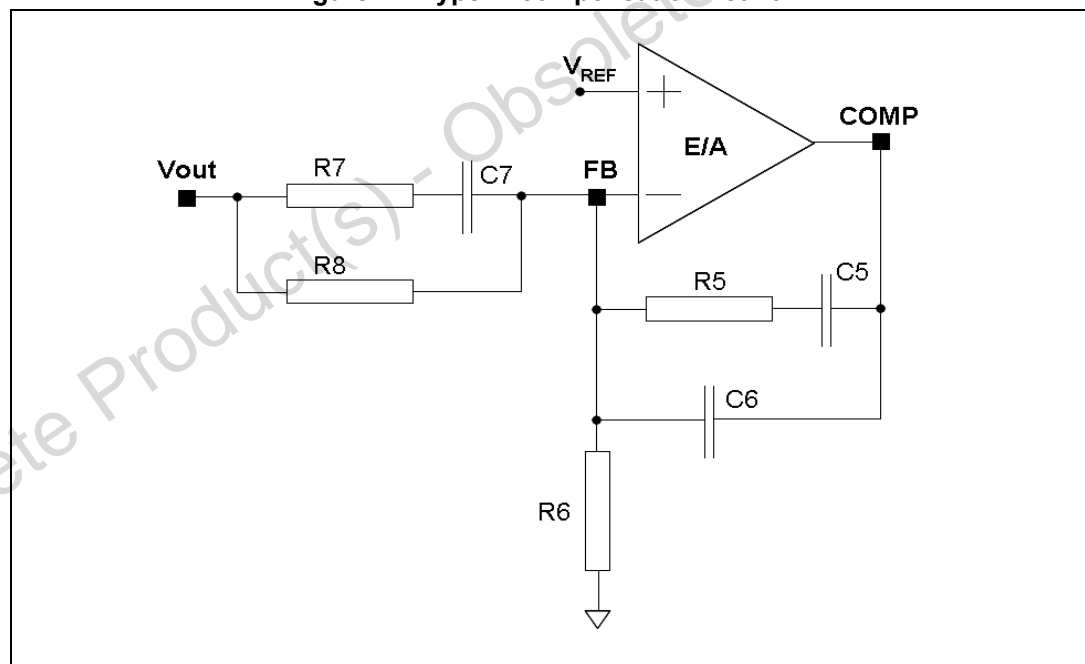
Figure 12. Type III compensation network
