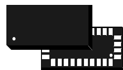
LGA-28L (4.4x7.5x1.1mm)
