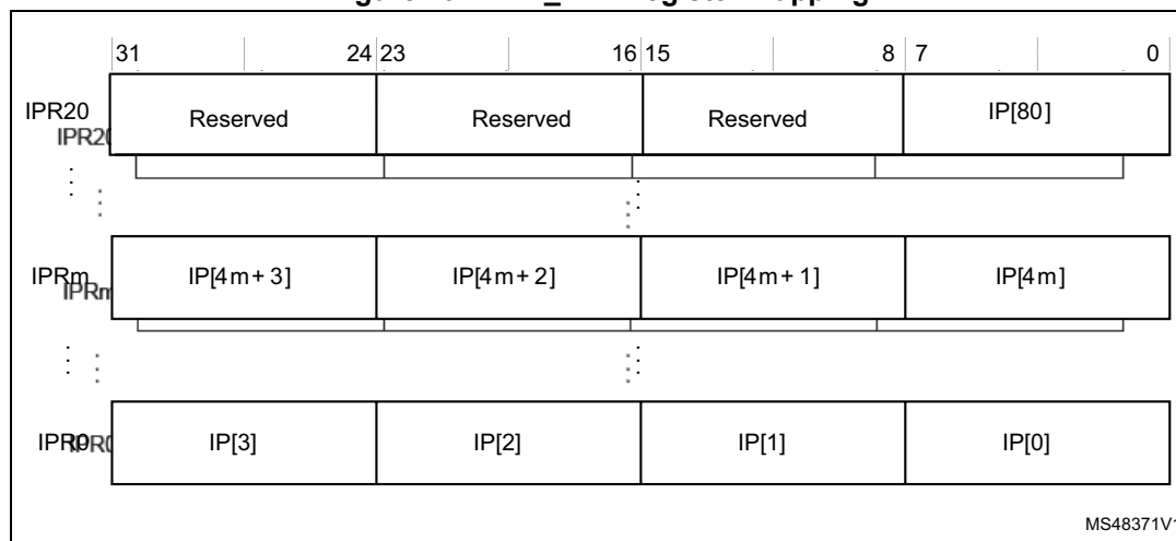
Figure 19. NVIC_IPRx register mapping
