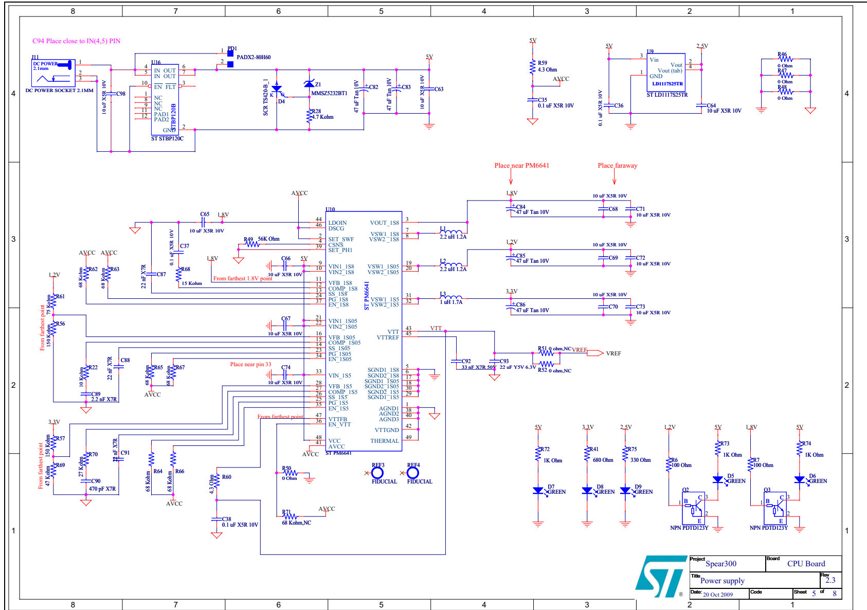
Figure 10. Power supply schematic
