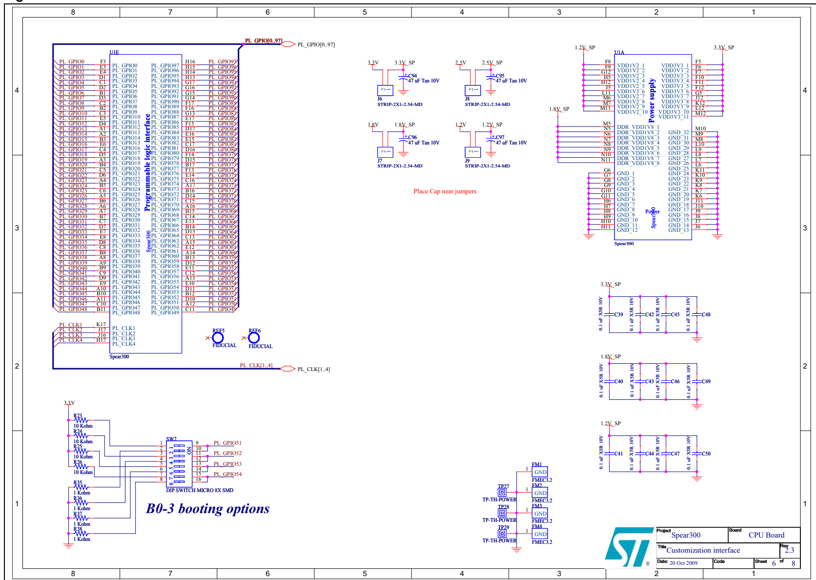
Figure 11. Customization interface schematic
