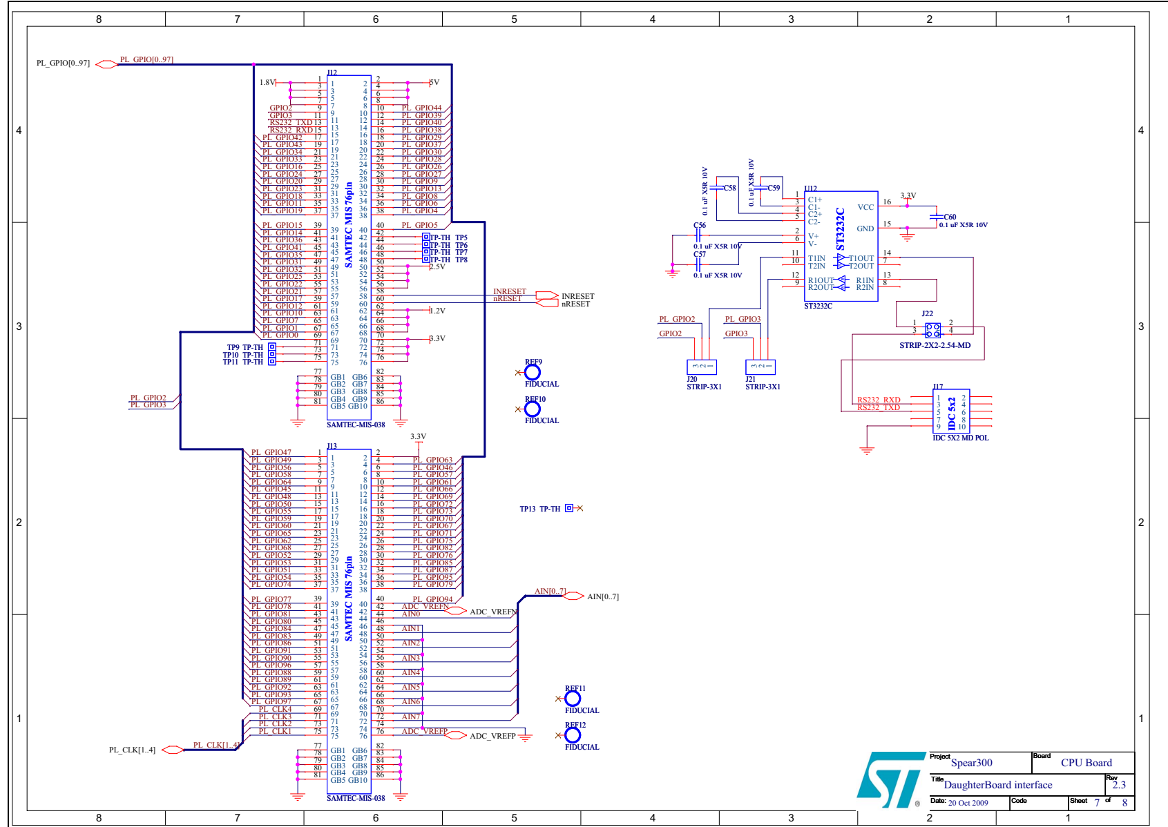
Figure 12. Daughterboard interface schematic
