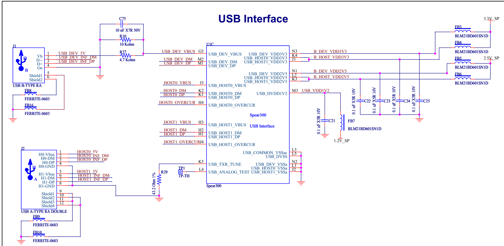
Figure 7. USB interface schematic
