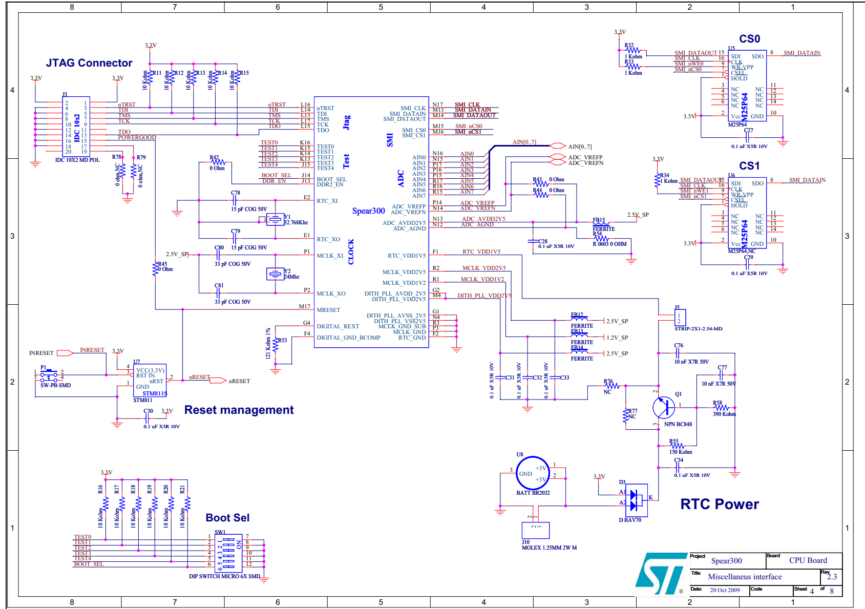
Figure 9. Miscellaneous interfaces schematic
