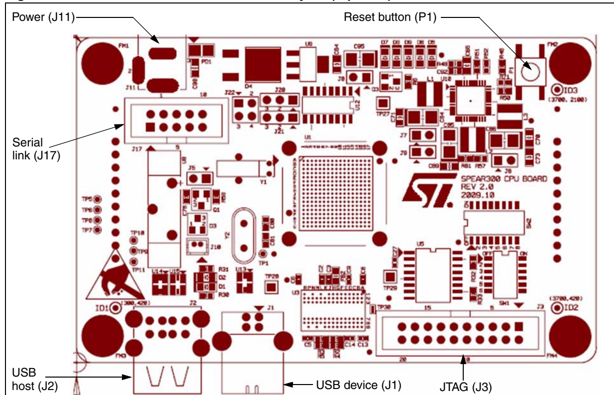
Figure 14. SPEAr320 CPU evaluation board layout (top view)
