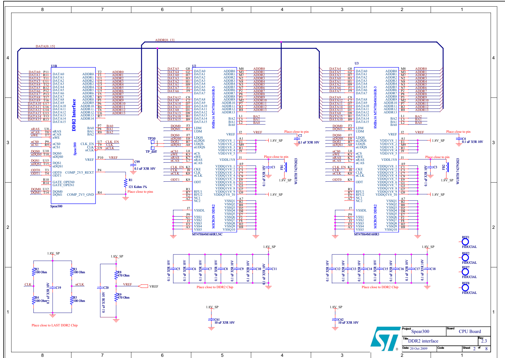
Figure 6. DDR interface schematic
