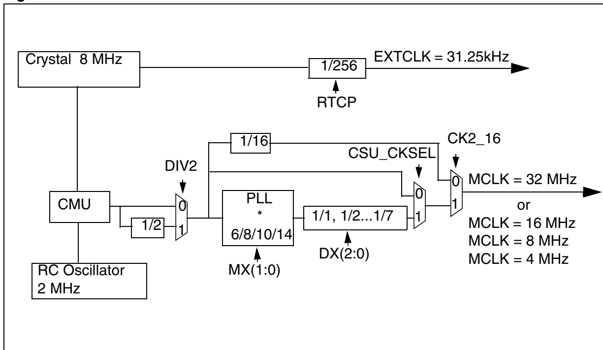
Figure 4. Clock Control
