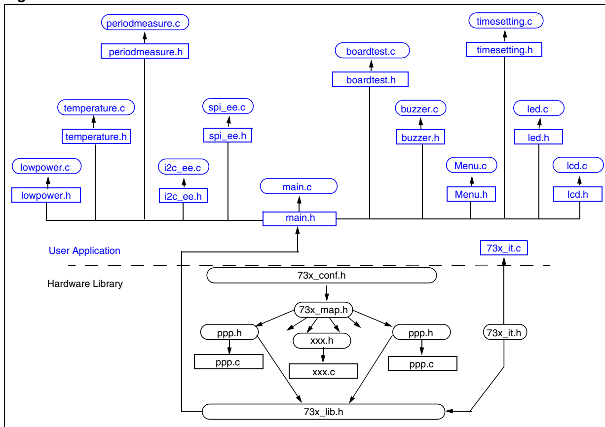
Figure 7. Software Architecture
