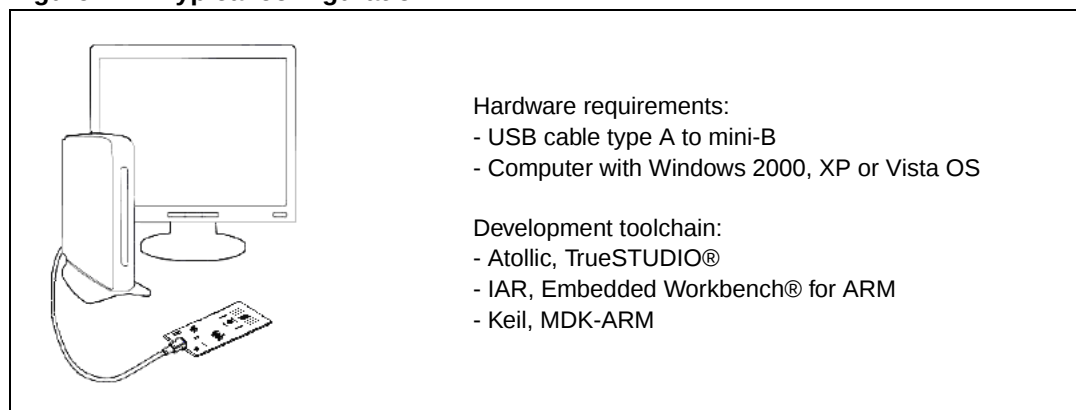
Figure 7. Typical configuration
