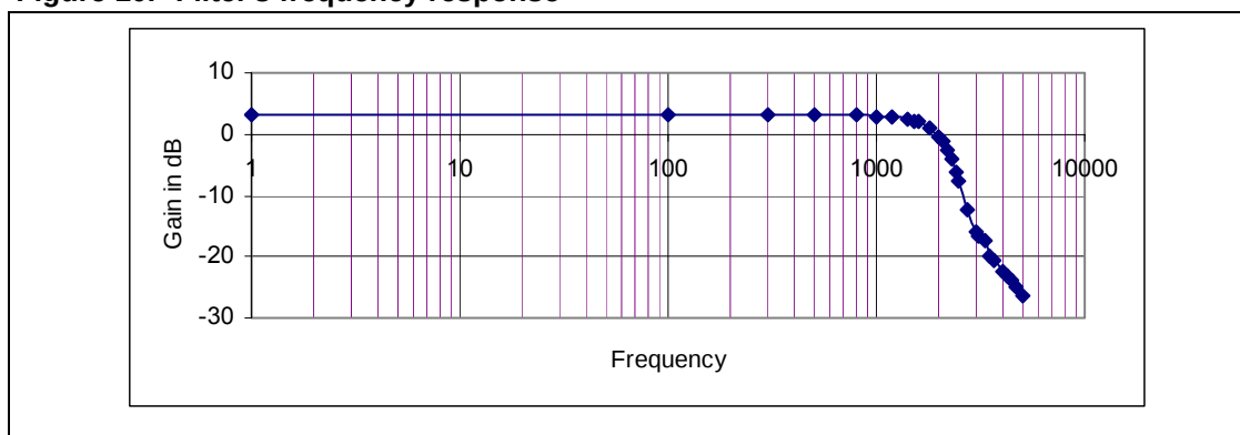
Figure 10. Filter's frequency response
