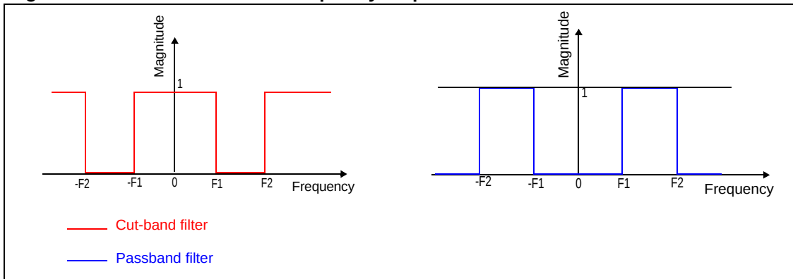
Figure 7. Ideal cut-band filter frequency response
