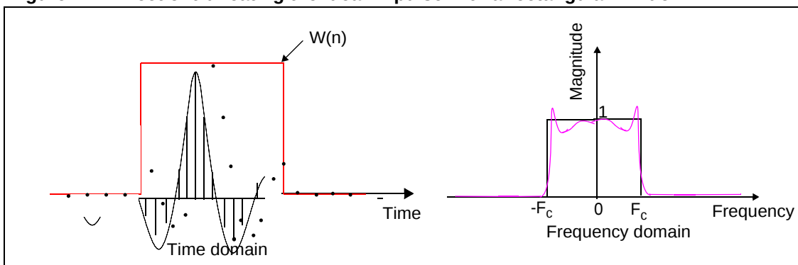
Figure 4. Effect of truncating the ideal impulse with a rectangular window
