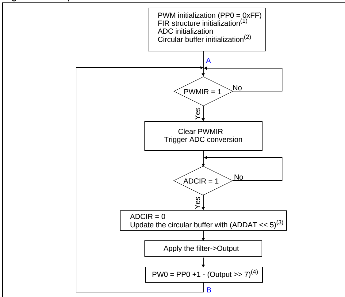
Figure 9. Low-pass filter flowchart
