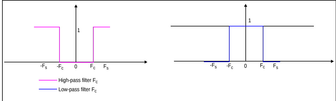
Figure 5. Ideal high-pass filter frequency response
