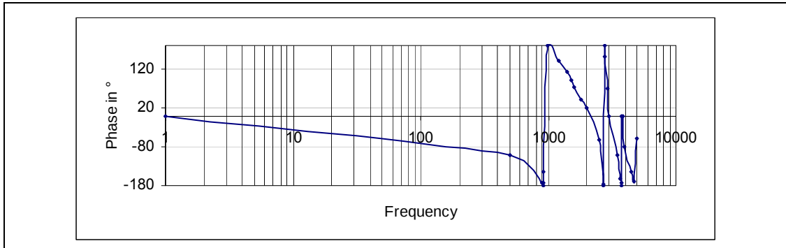
Figure 11. Phase response
