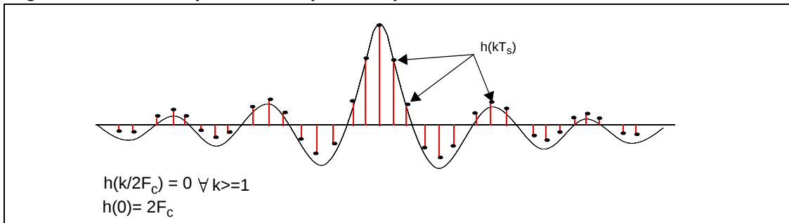
Figure 3. Ideal low-pass filter impulse response
