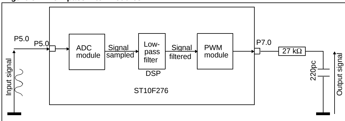
Figure 8. Low-pass filter modules
