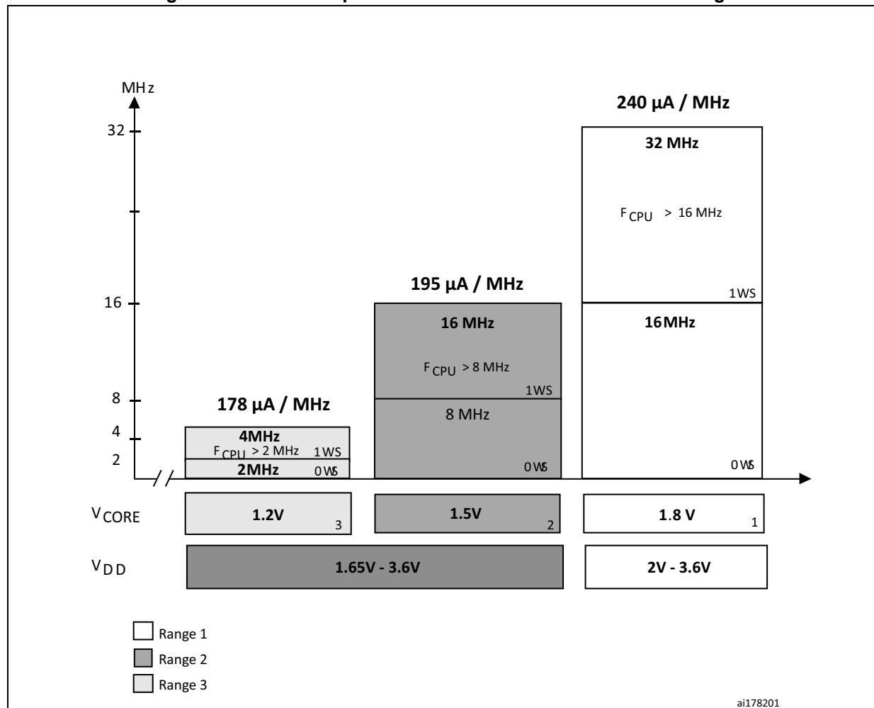
Figure 1. STM32L1xx performance versus VDD and VCore range
