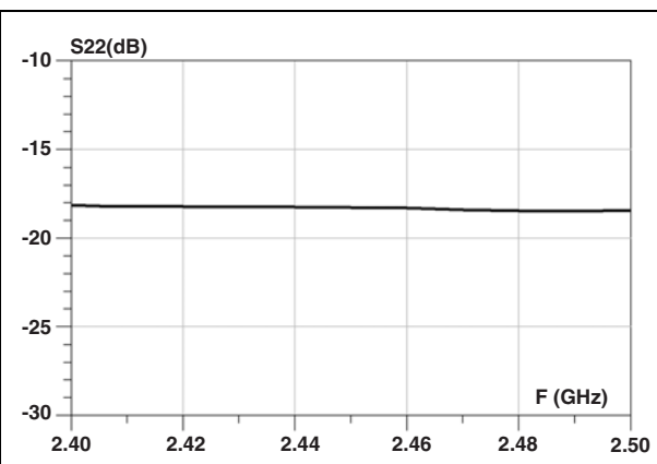
Figure 7. 2 G return loss ( T_{amb} = 25\text{ °C} )
