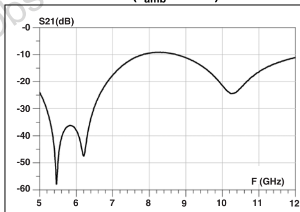
Figure 6. 2 G attenuation in high frequency band ( T_{amb} = 25\text{ °C} )
