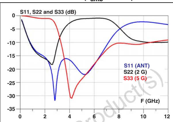
Figure 3. 2 G, 5 G and antenna reflection coefficient ( T_{amb} = 25\text{ °C} )
