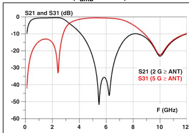
Figure 2. 2 G and 5 G forward transmission ( T_{amb} = 25\text{ °C} )
