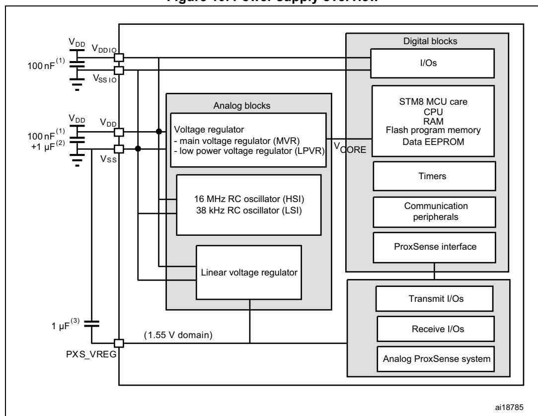
Figure 10. Power supply overview
