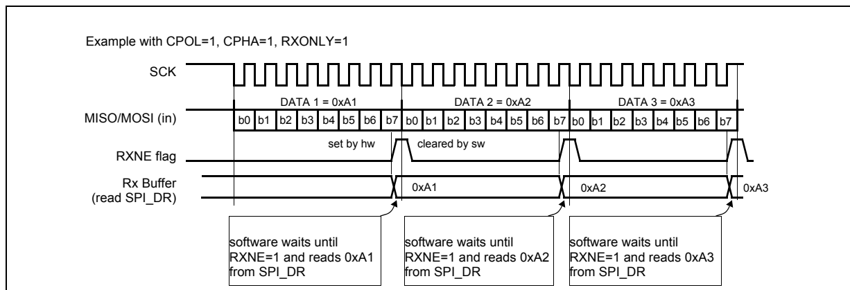
Figure 79. RXNE behavior in receive-only mode (BDM = 0 and RXONLY = 1). Case of continuous transfers
