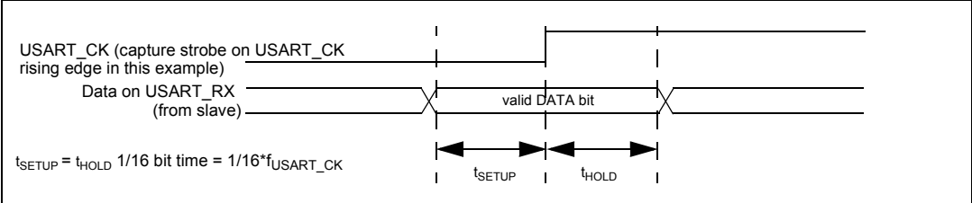
Figure 93. RX data setup/hold time
