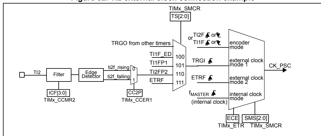
Figure 32. TI2 external clock connection example
