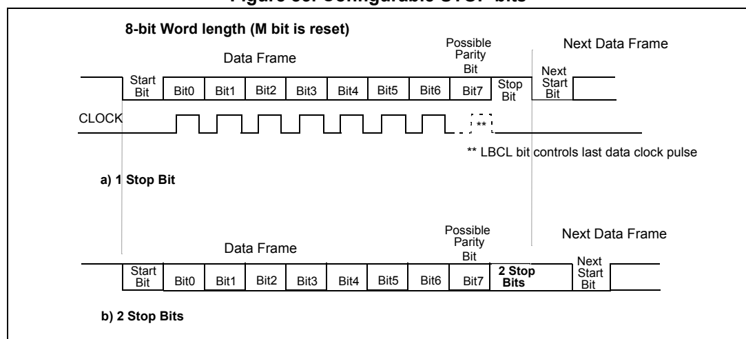
Figure 83. Configurable STOP bits
