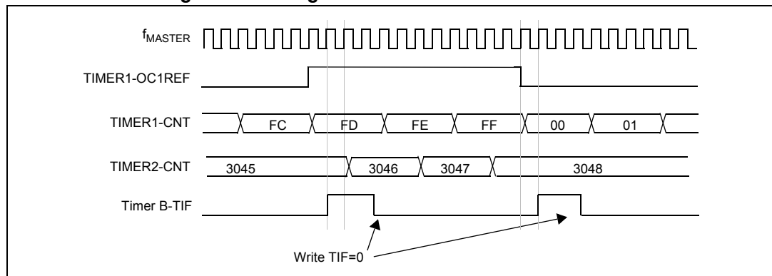
Figure 43. Gating Timer B with OC1REF of Timer A
