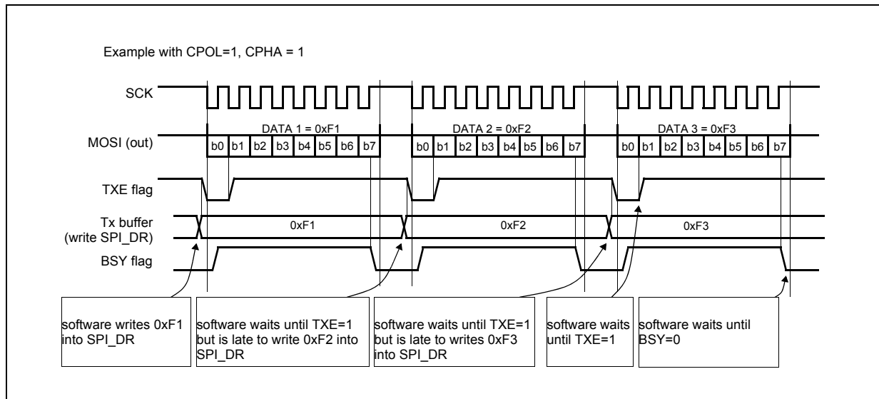
Figure 80. TXE/BSY behavior when transmitting (BDM = 0 and RXLON = 0). Case of discontinuous transfers
