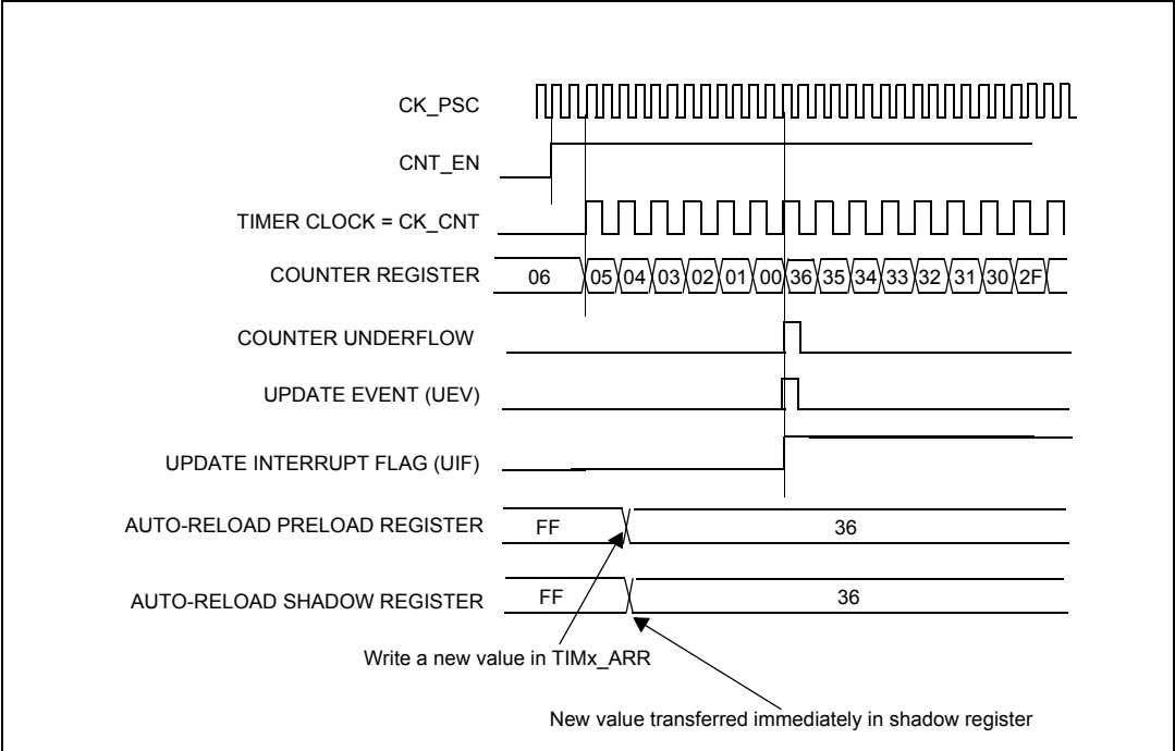
Figure 26. Counter update when ARPE=0 (ARR not preloaded) with prescaler = 2
