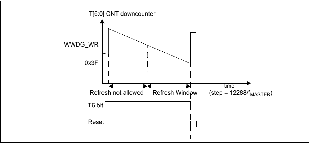
Figure 17. Window watchdog timing diagram
