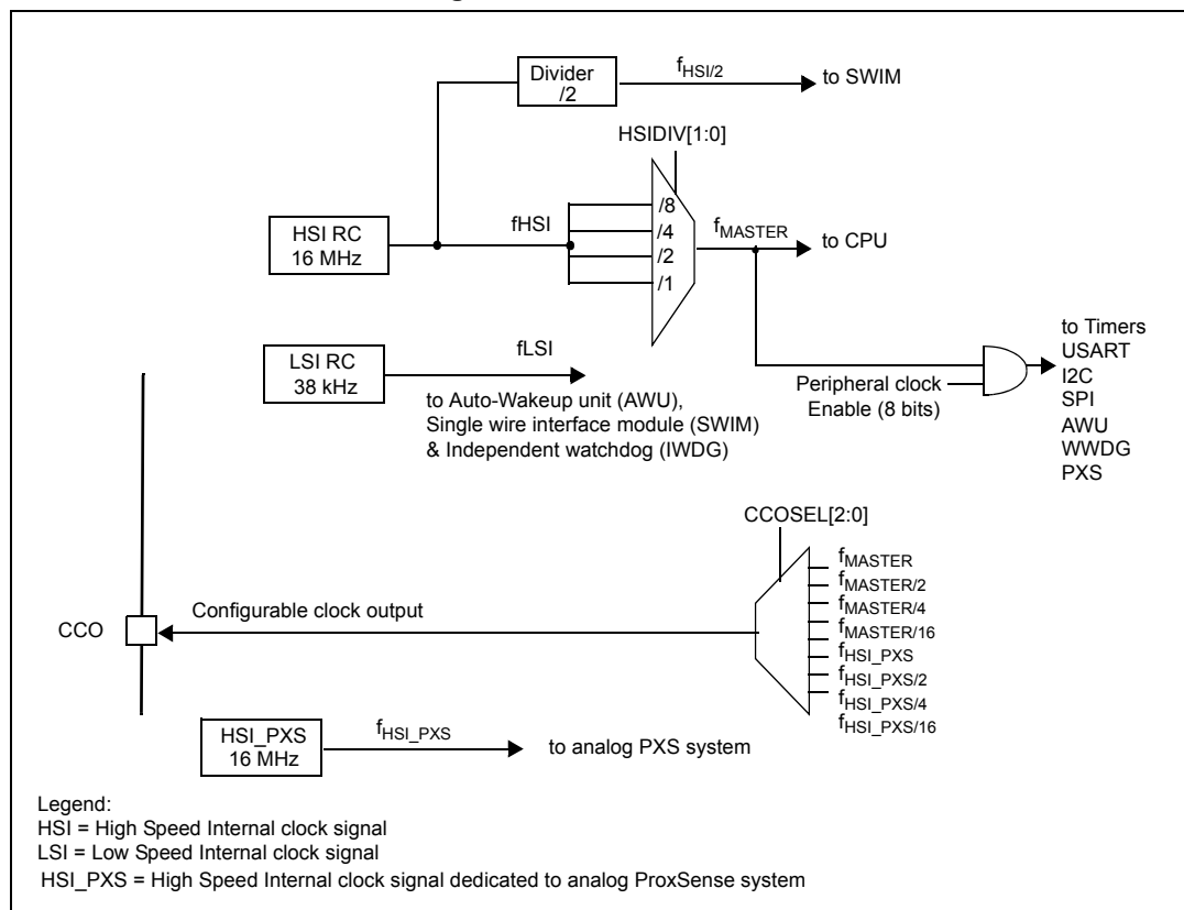
Figure 12. Clock structure
