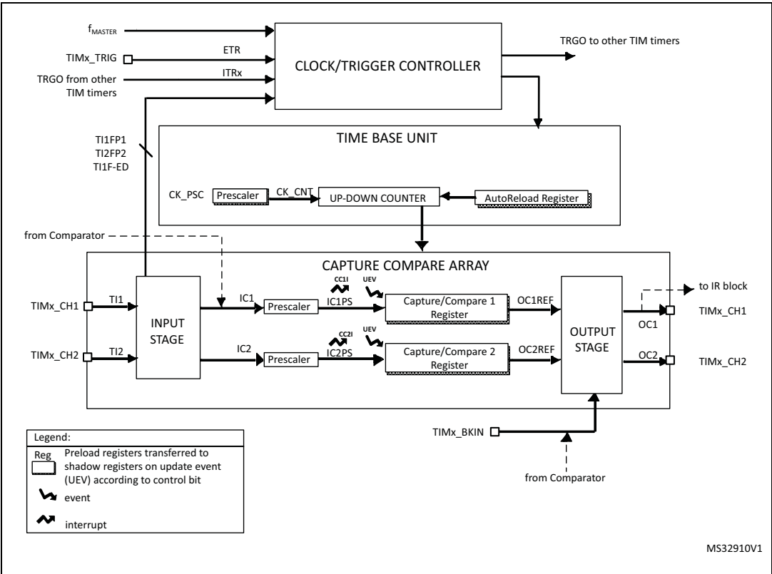
Figure 19. TIMx general block diagram
