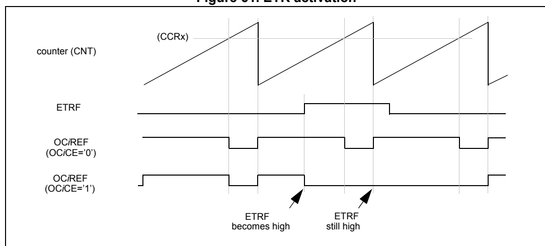
Figure 61. ETR activation
