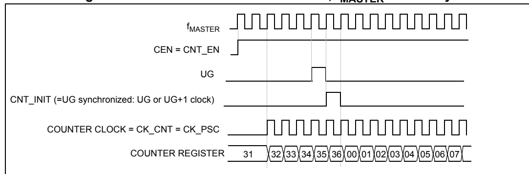
Figure 31. Control circuit in normal mode, f_{\text{MASTER}} divided by 1
