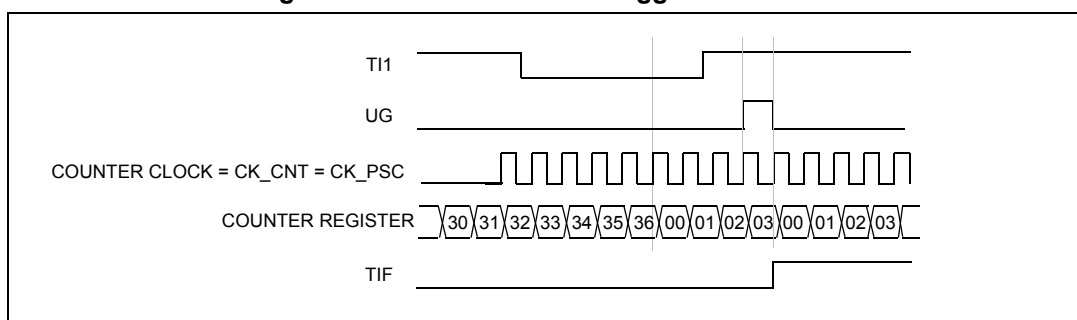
Figure 37. Control circuit in trigger reset mode
