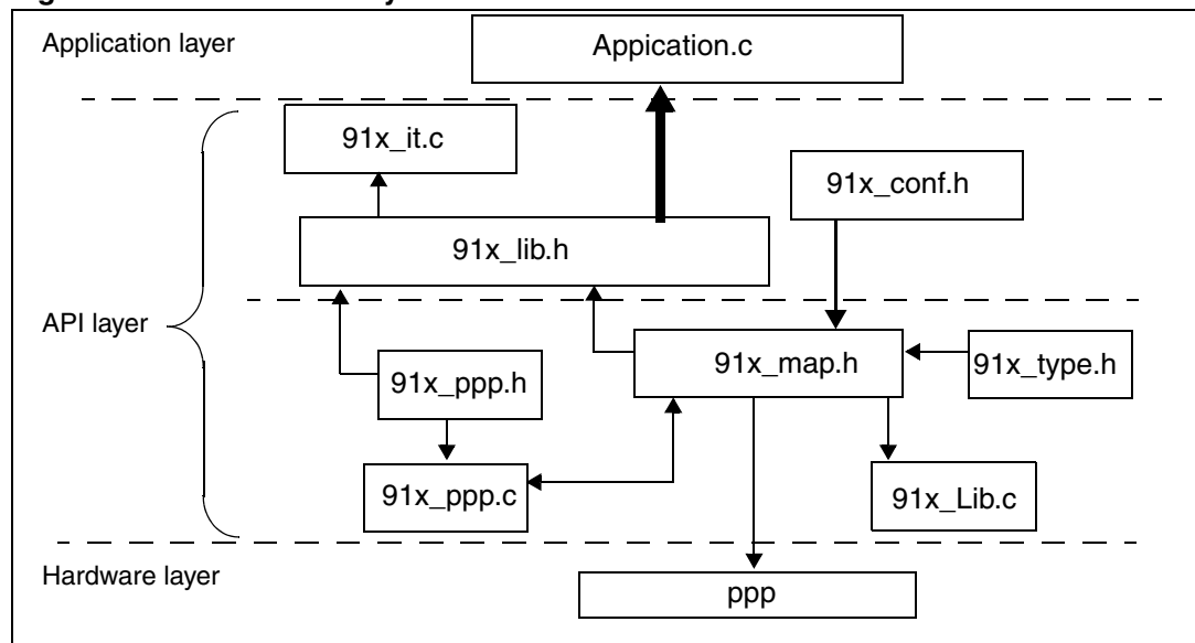
Figure 2. Firmware library file architecture
