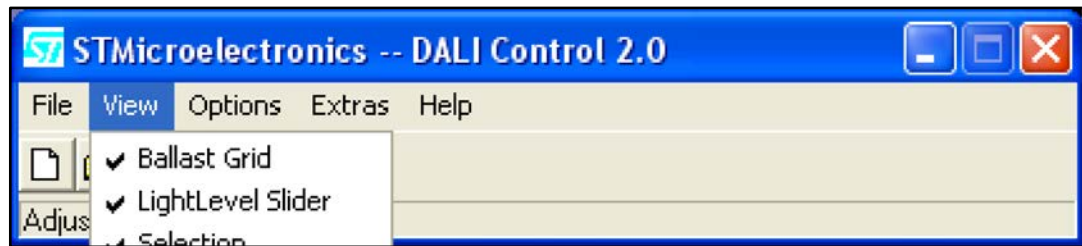
Figure 12: Main window
