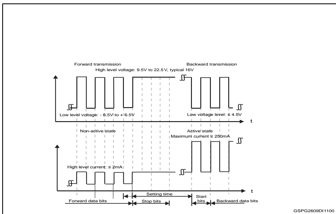
Figure 2: Voltage and currents on the DALI bus
