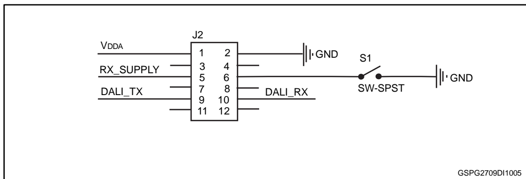
Figure 7: Schematic of connector J2
