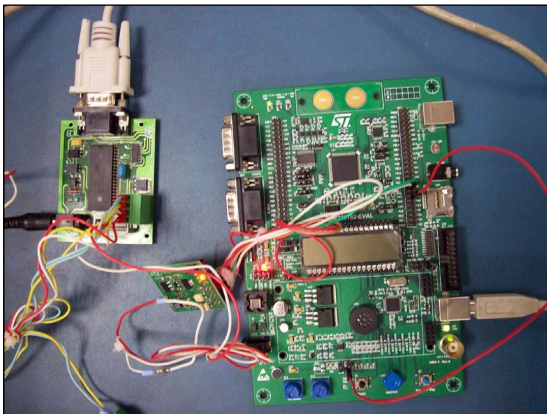
Figure 11: Complete DALI setup
