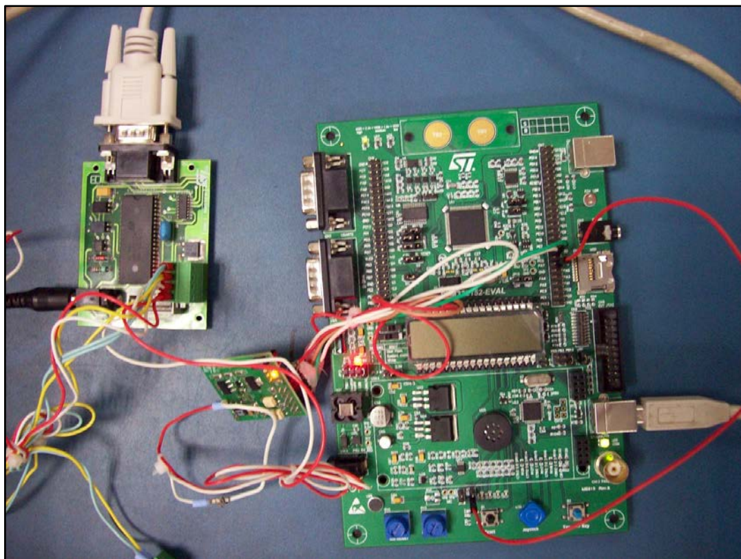
Figure 5: Hardware for testing DALI: STM32L EVAL board with DALI transceiver board and ST7 DALI master board
