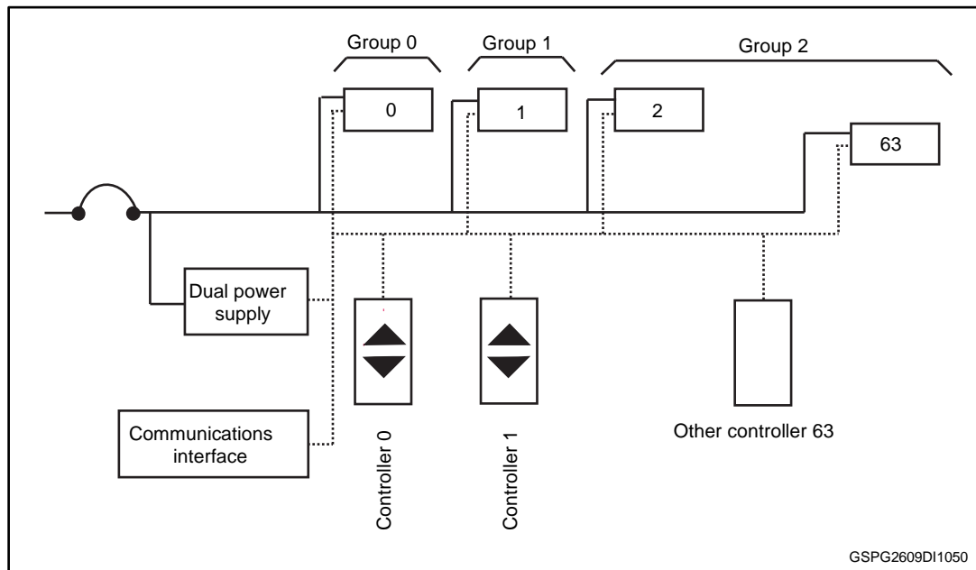
Figure 1: Example of DALI device connections
