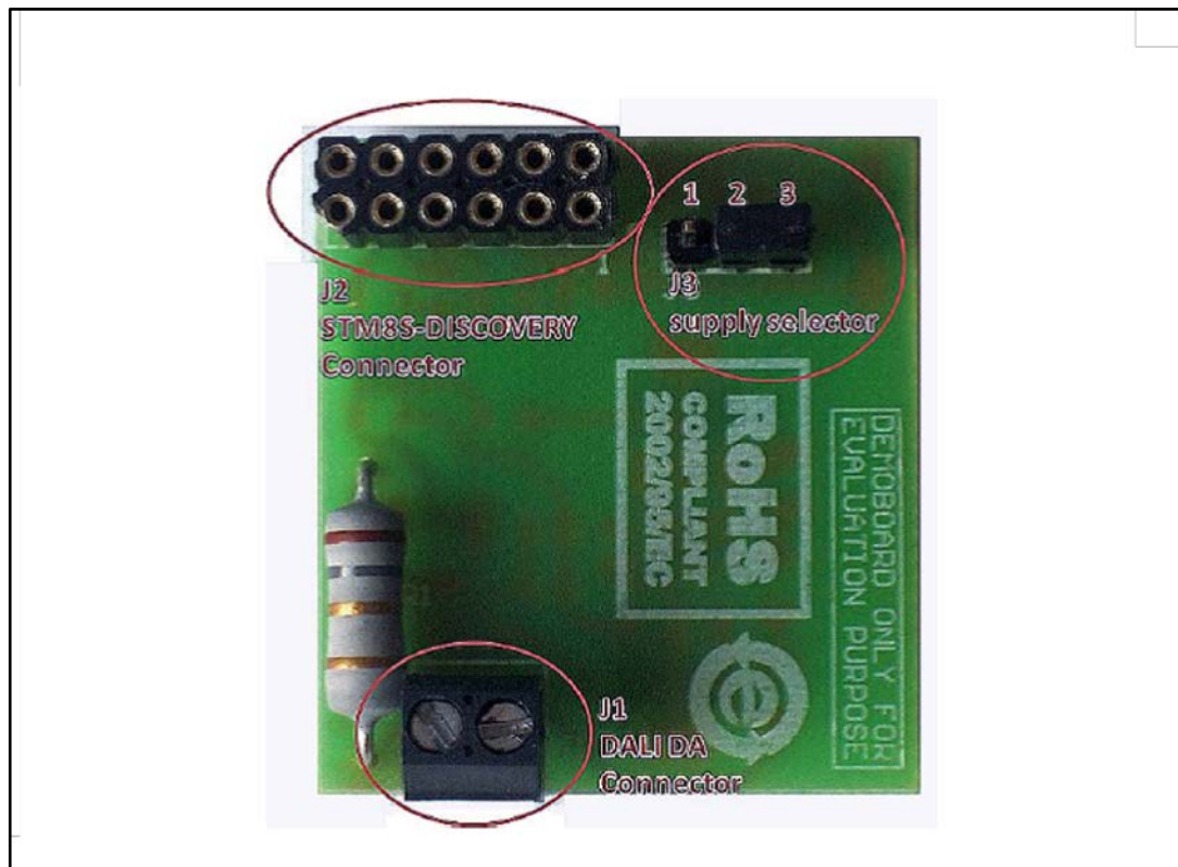
Figure 6: Bottom side connectors
