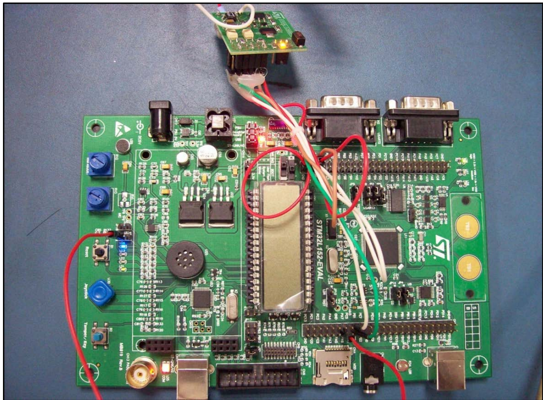
Figure 9: Slave Device setup (STEVAL-ILM001V1 and STM32L152-EVAL board)
