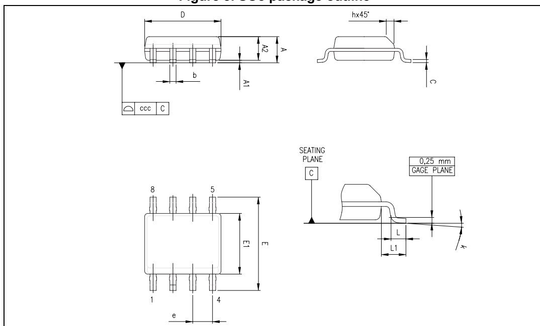
Figure 8. SO8 package outline
