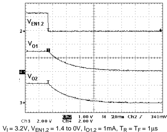
Figure 17: TURN-OFF
