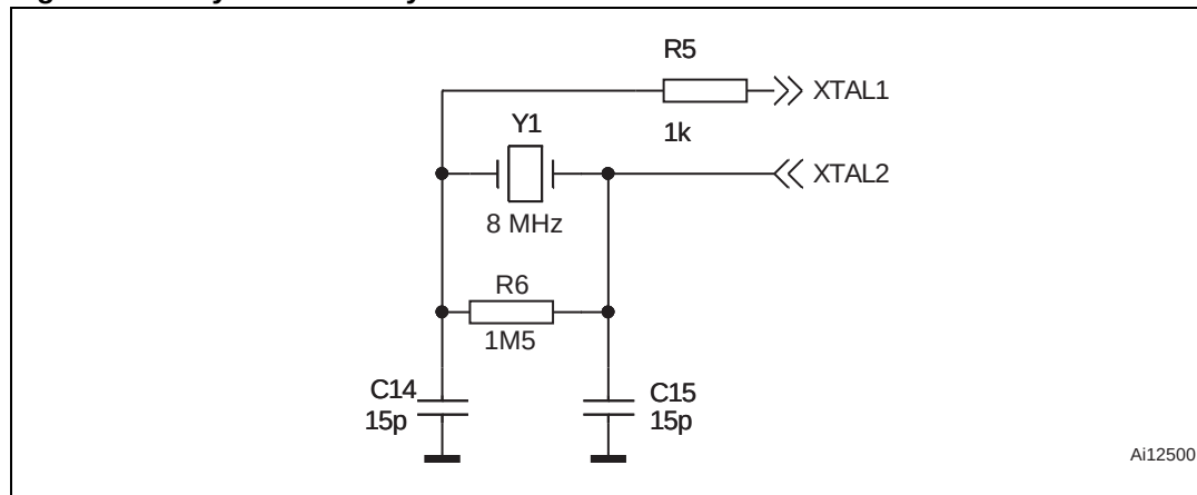
Figure 16. Crystal assembly
