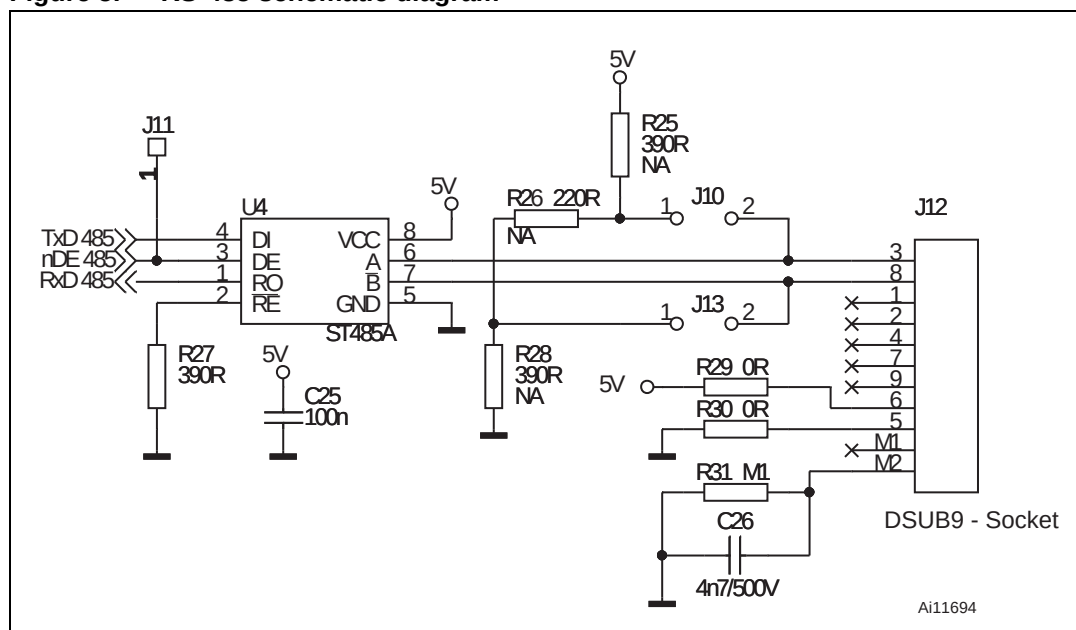
Figure 5. RS-485 schematic diagram
