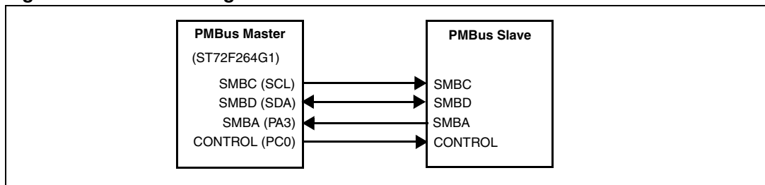
Figure 1. Interface diagram
