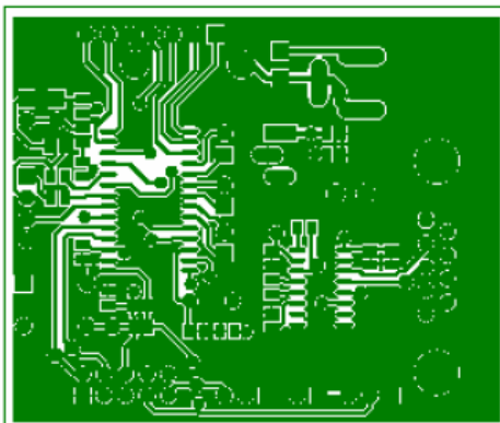
Figure 27. Top view layout of the demonstration board
