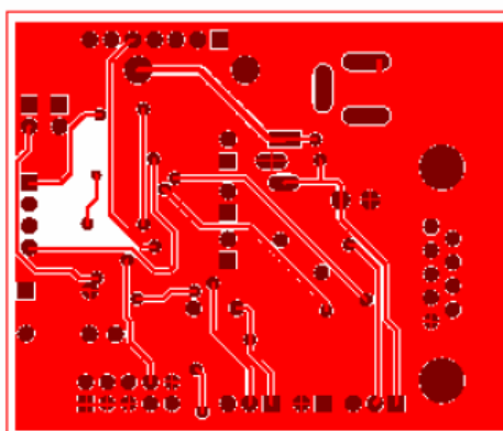
Figure 28. Bottom view layout of the demonstration board
