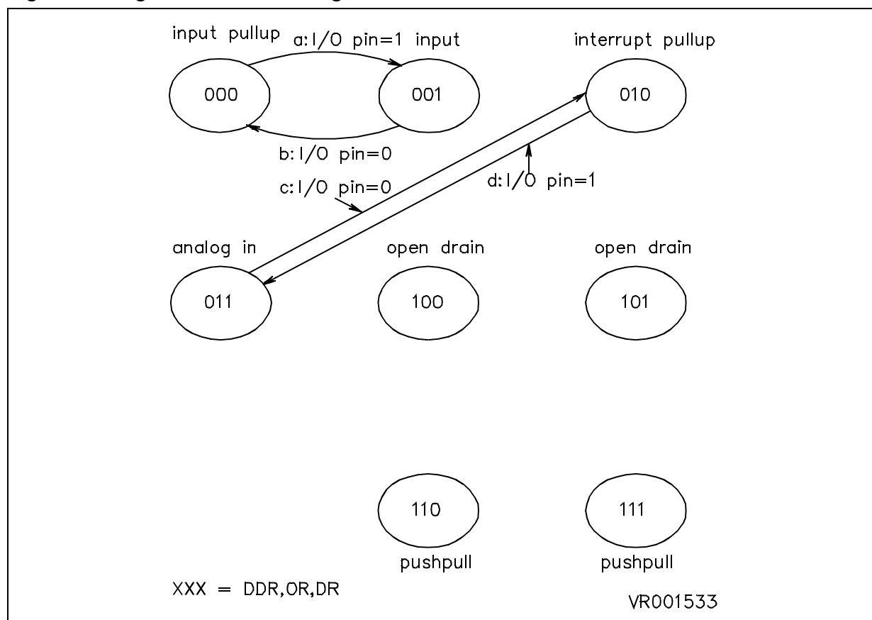
Figure 8. Diagram for I/O data register False transitions
