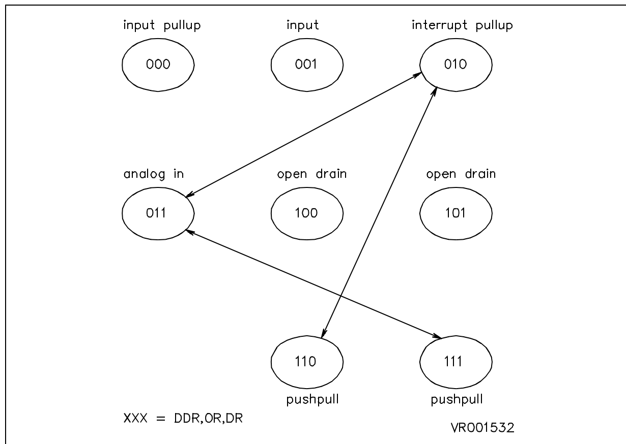
Figure 7. Diagram for risky transitions
