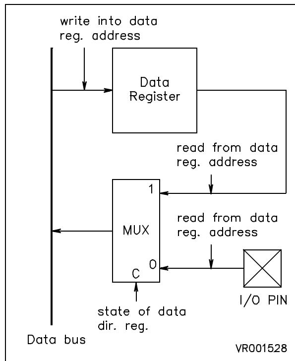
Figure 3. Read multiplexing
