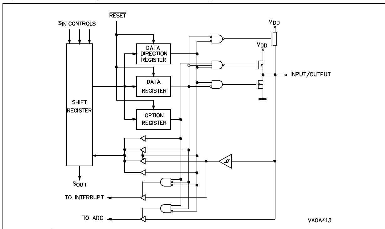
Figure 1. ST62XX I/O port structure with A/D input
