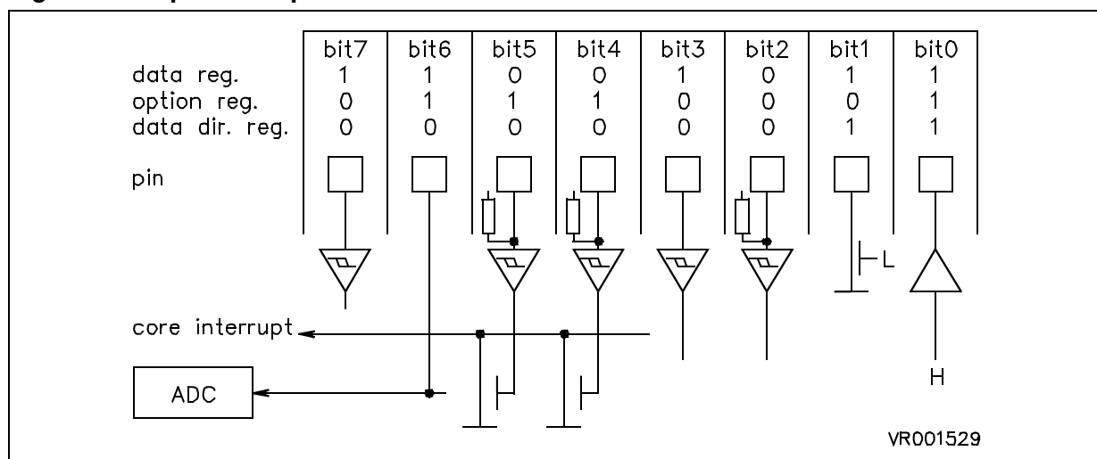
Figure 4. I/O port with pins in different functions
