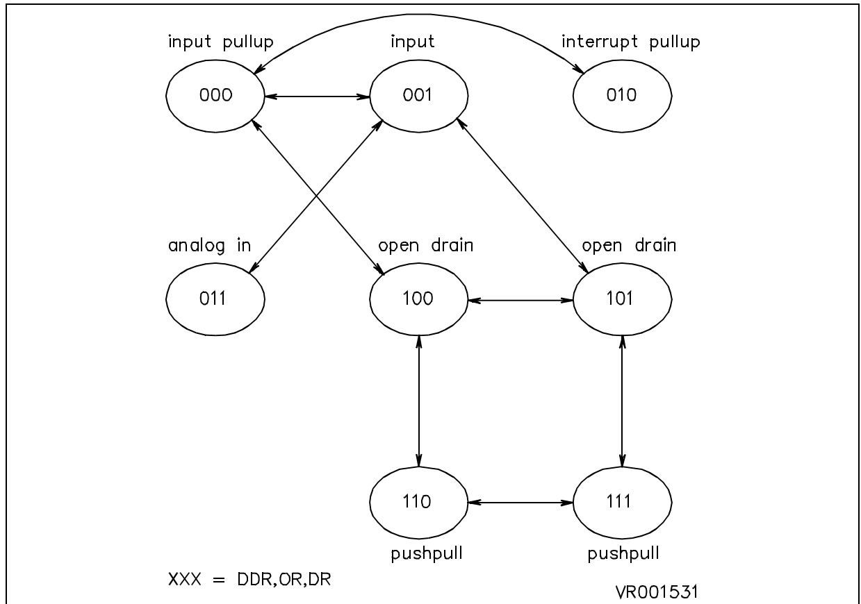
Figure 6. Diagram for safe transitions
