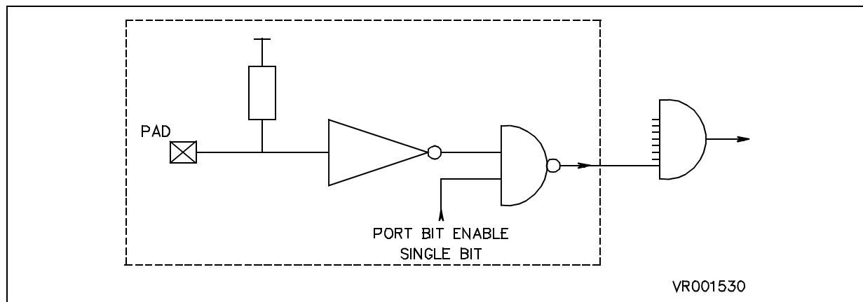
Figure 5. Interrupt schematic for one I/O pin
