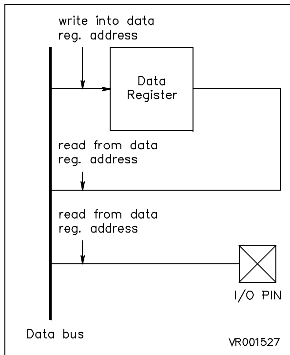
Figure 2. Data register access
