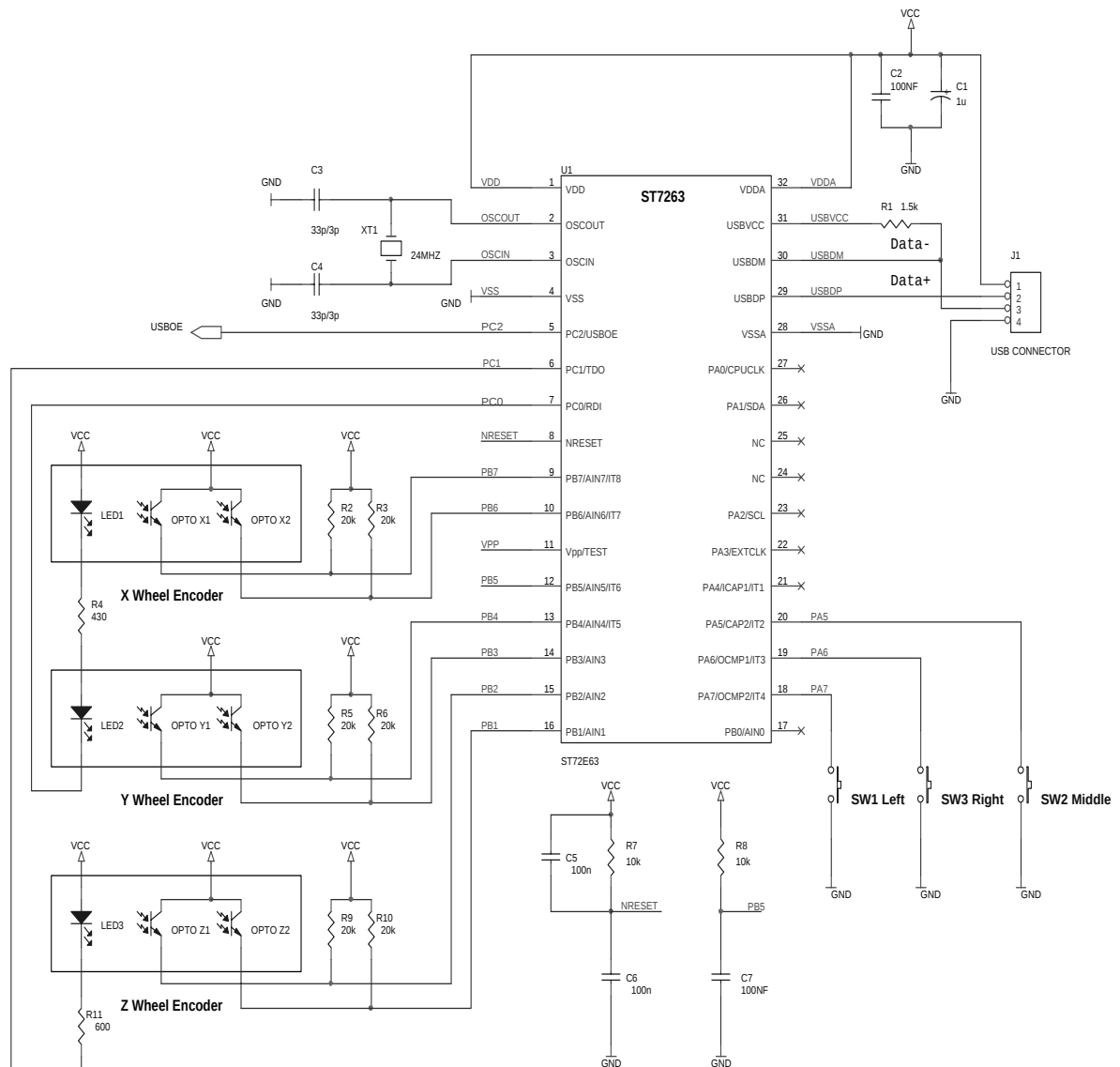
Figure 4. Hardware Implementation
