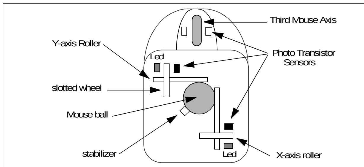
Figure 1. Mouse mechanical hardware
