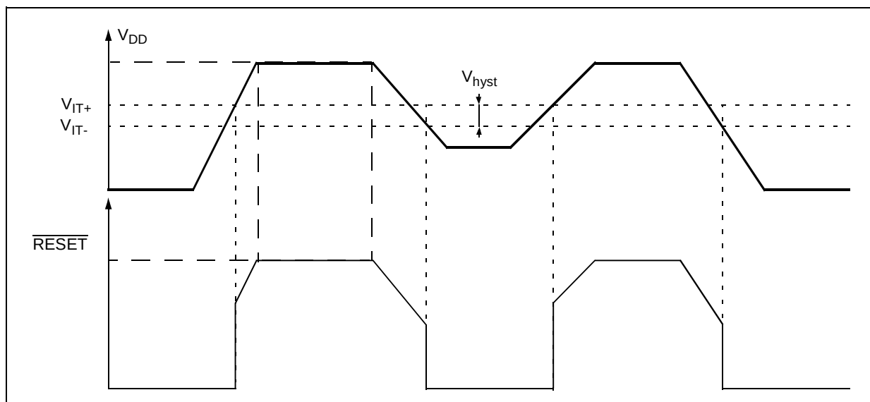
Figure 1. Low Voltage Detector Reset
