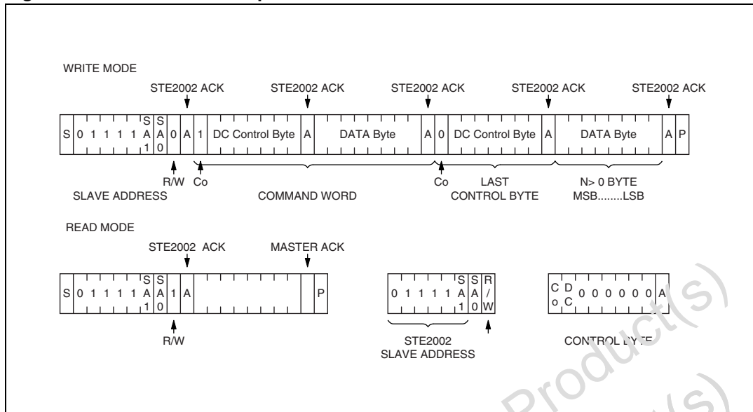
Figure 30. Communication protocol
