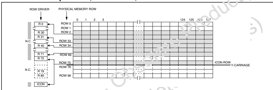
Figure 20. Memory rows vs. row drivers mapping with MUX65, Y-CARRIAGE=6, scroll pointer=3, icon mode=1,
