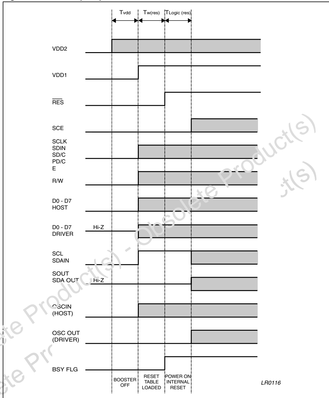
Figure 41. Power-up sequence
