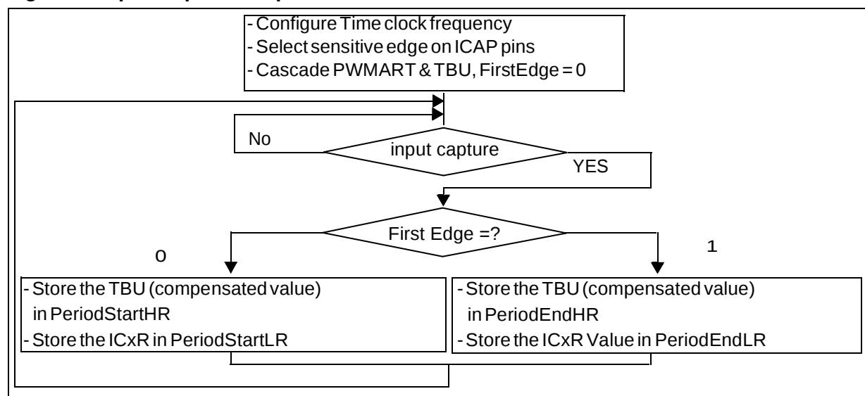
Figure 7. Input Capture Sequence
