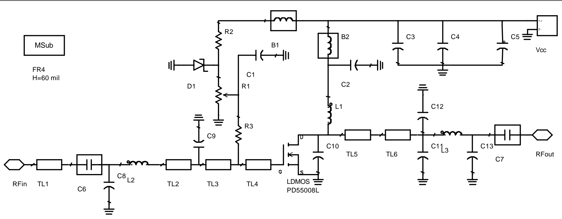
DB-55008L-470 schematic
