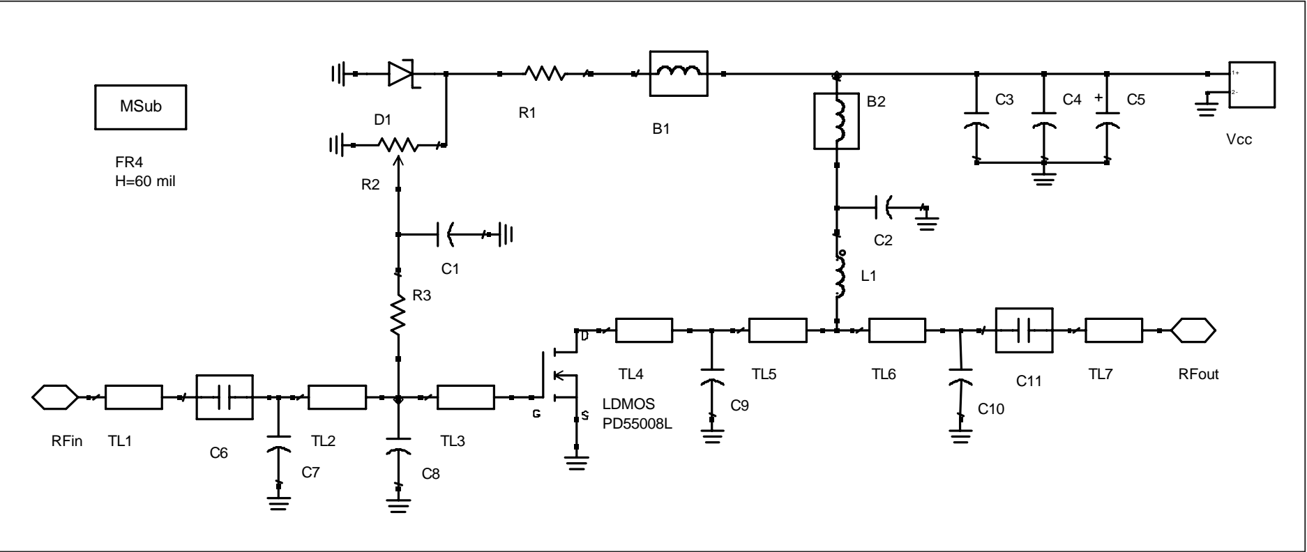
DB-55008L-960 schematic
