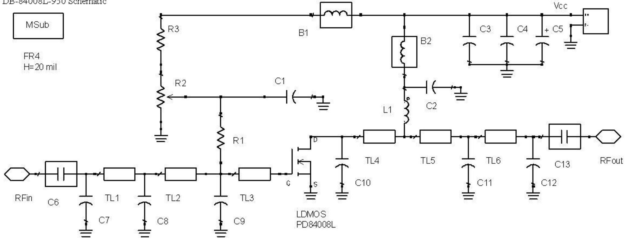
DB-84008L-950 Schematic
