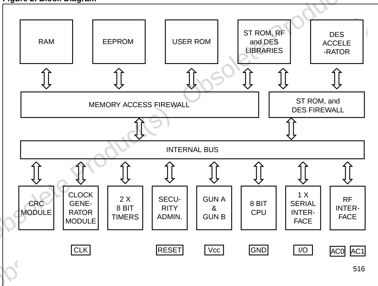
Figure 2. Block Diagram
