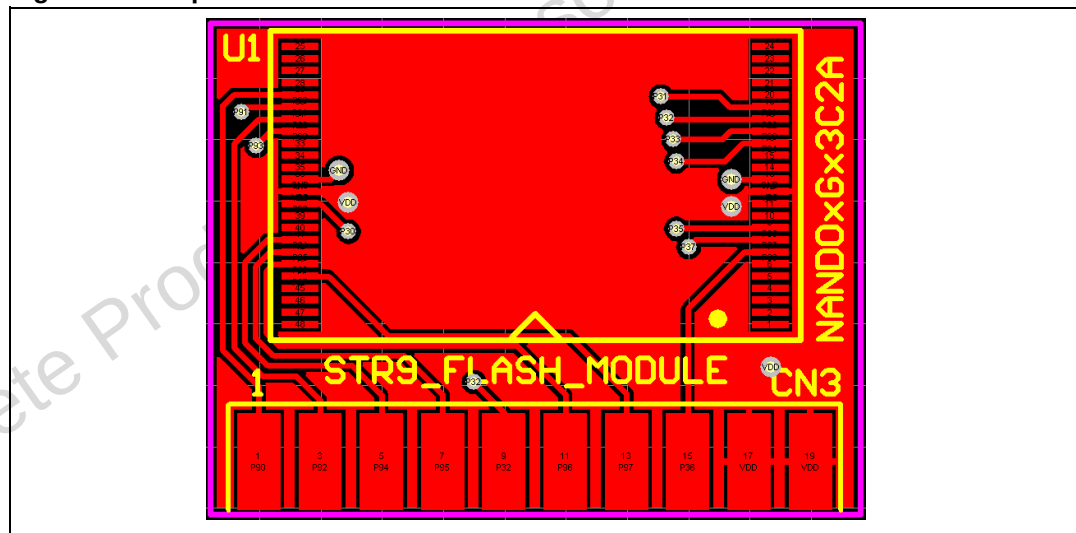
Figure 5. Top view
