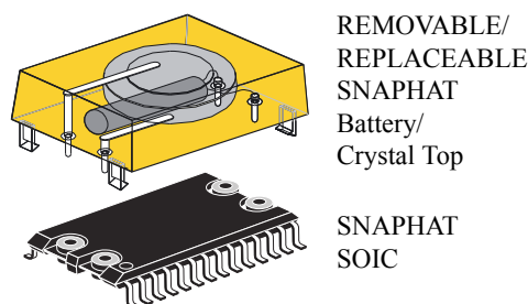
Figure 3. SNAPHAT SOIC package
