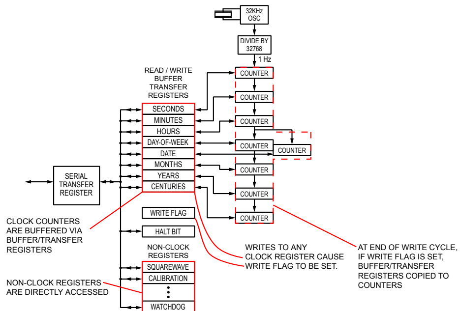
Figure 13. Clock and non-clock registers
