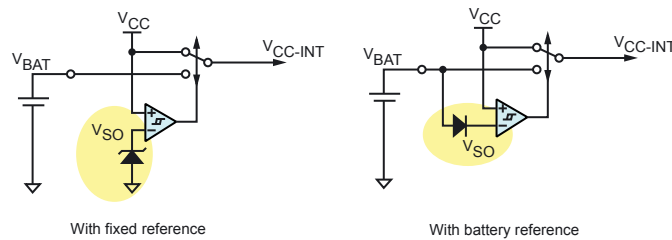
Figure 9. Typical switchover circuits
