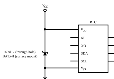
Figure 8. Undershoot protection
