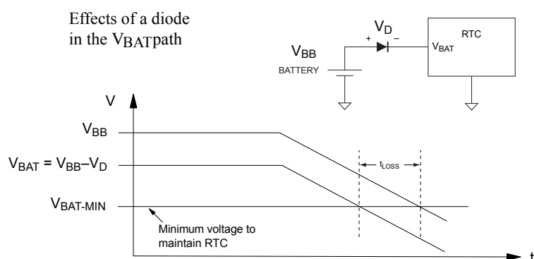
Figure 2. Effects of a diode in the V_{BAT} path
