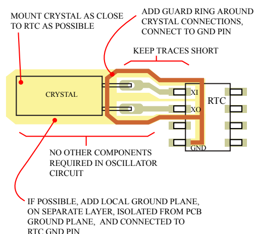
Figure 5. Layout considerations
