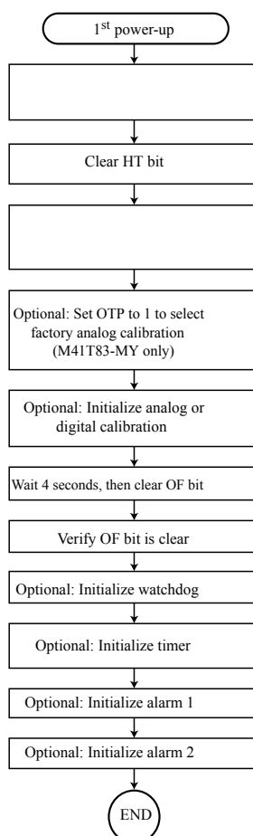
Figure 15. First power-up
