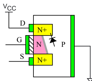
Figure 7. Typical parasitic diode
