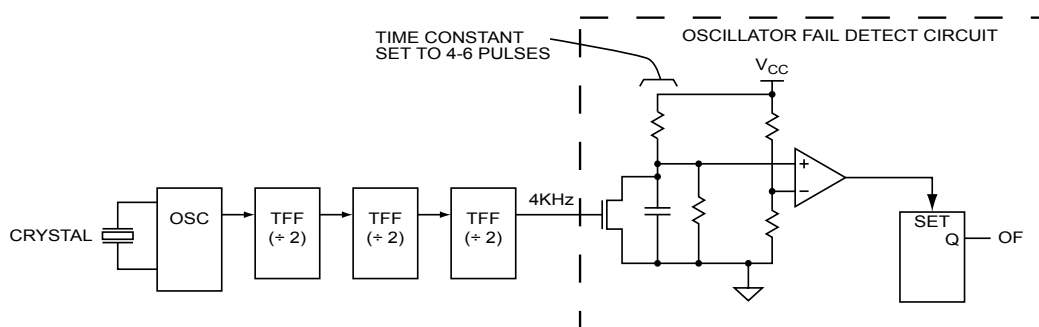
Figure 11. Oscillator fail detect circuit
