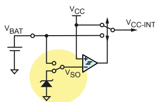
Figure 10. Switchover circuit
