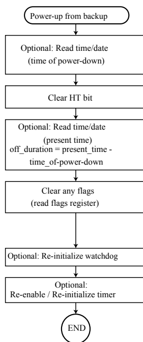
Figure 16. Power-up from backup
