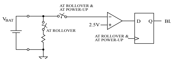
Figure 12. Battery monitor function
