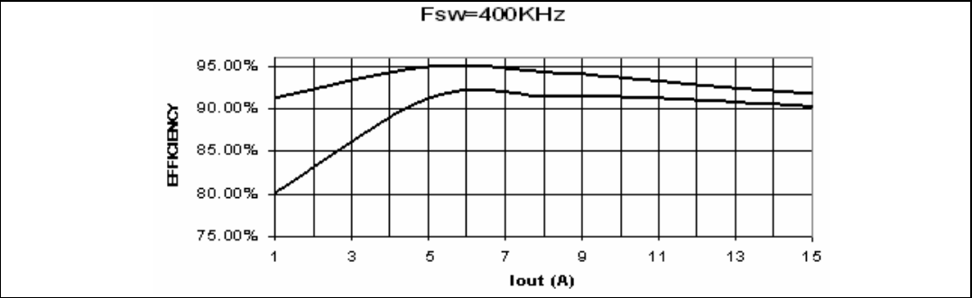
Figure 2. Demoboard efficiency
