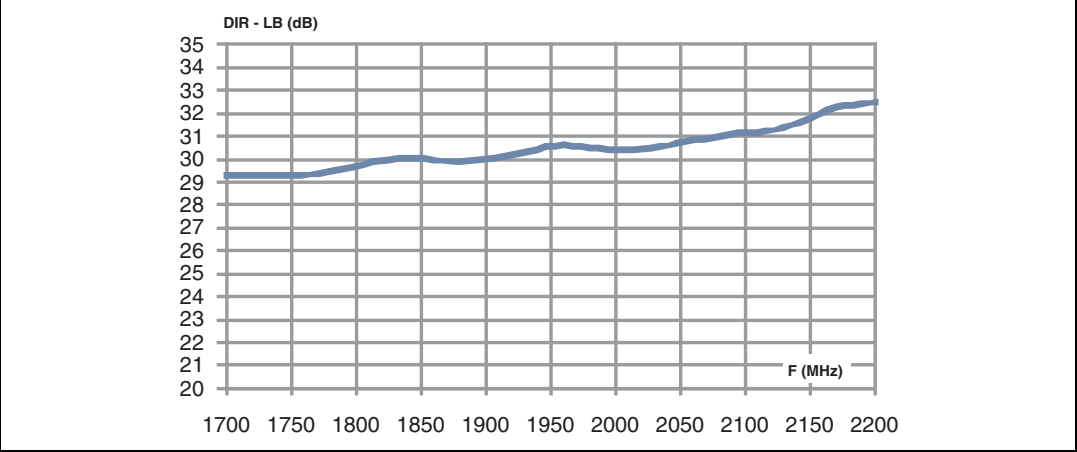
Figure 7. High band path directivity
