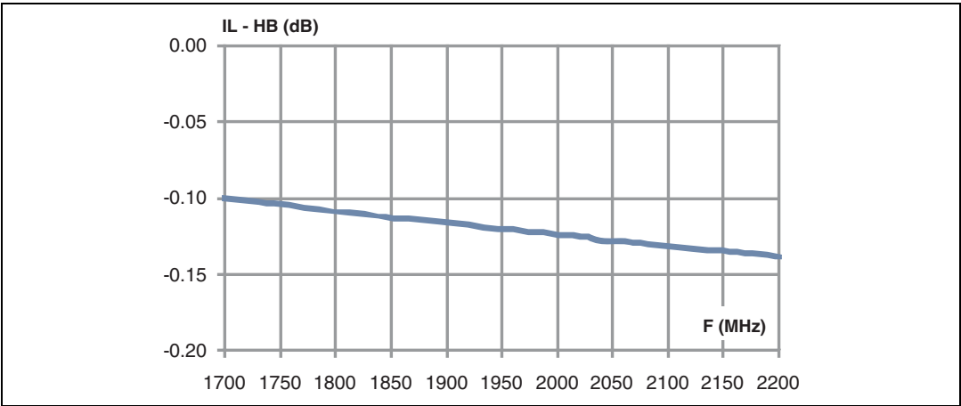
Figure 3. High band path insertion loss
