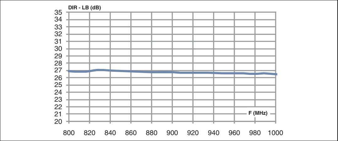
Figure 6. Low band path directivity
