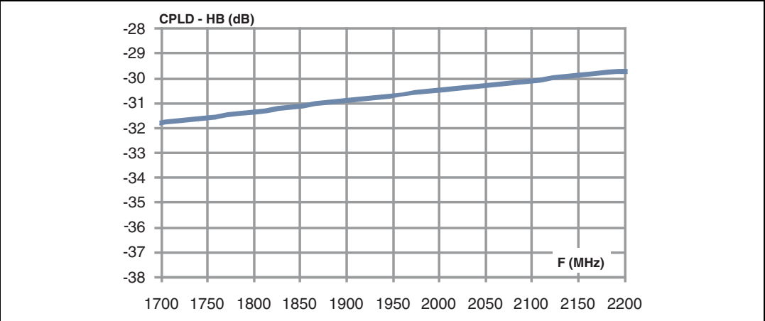
Figure 5. High band path coupling factor
