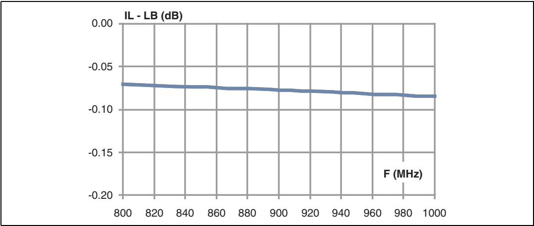
Figure 2. Low band path insertion loss
