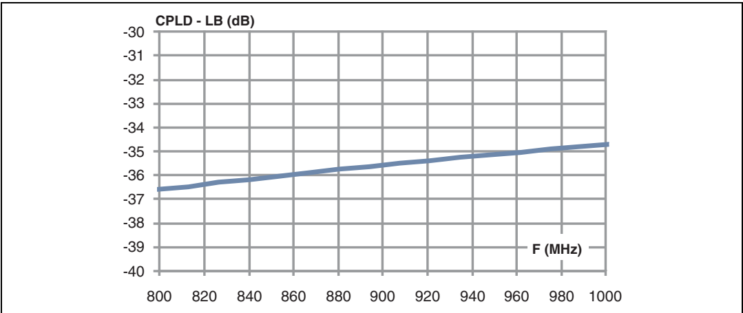
Figure 4. Low band path coupling factor
