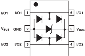
SOT666
