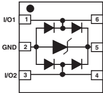
μQFN 6 leads
