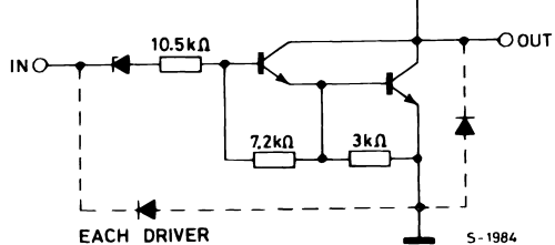
ULN2002 (each driver)
