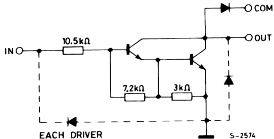
ULN2004 (each driver)
