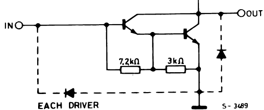
ULN2001 (each driver)
