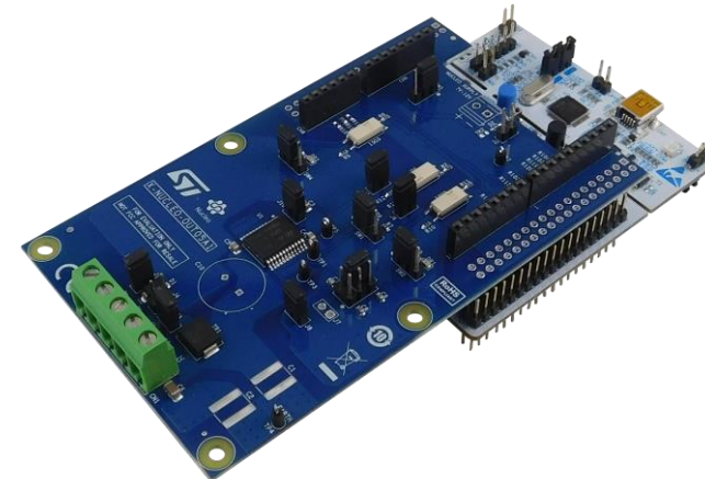
NUCLEO stacked solution
