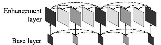
Fig. 2. Multi-layer structure with additional inter-layer prediction for enabling spatial scalable coding.
