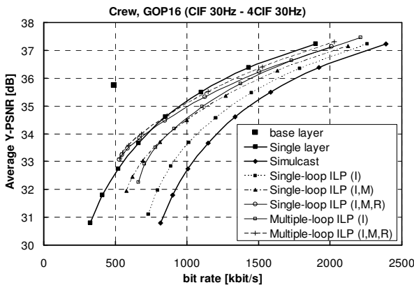
Fig. 4. Efficiency analysis of the inter-layer prediction concepts in SVC for different sequences and prediction structures. The rate-distortion point for the
