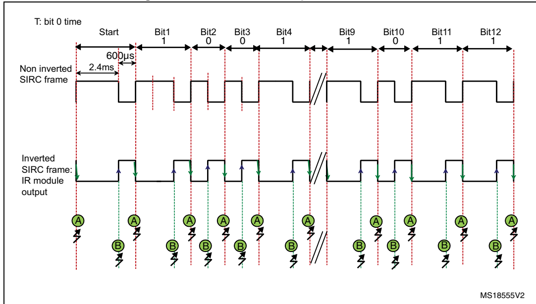
Figure 21. SIRC frame reception mechanism
