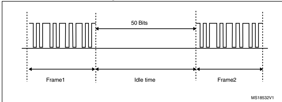
Figure 3. RC5 idle time
