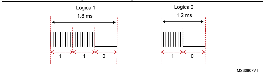
Figure 14. SIRC logical bit conversion
