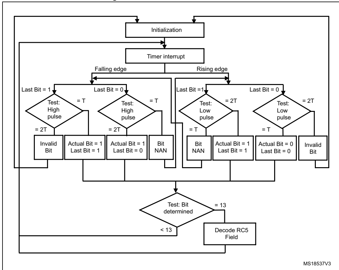
Figure 20. RC5 solution flowchart
