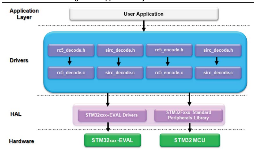
Figure 23. Application layer architecture
