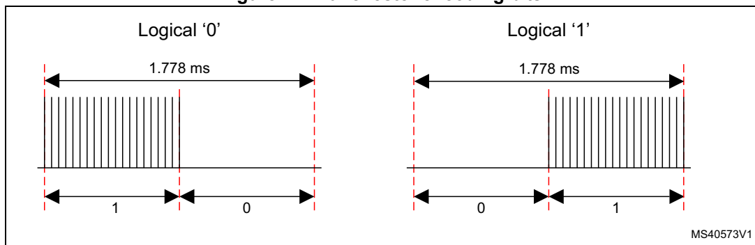
Figure 12. Manchester encoding bits
