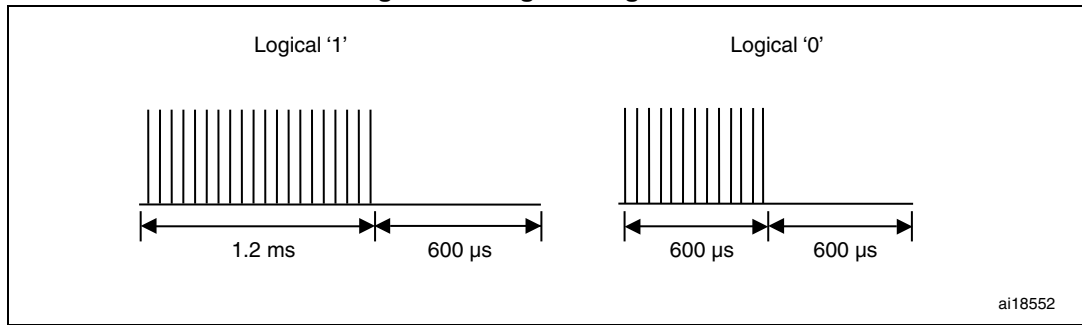
Figure 4. Length of logical bits
