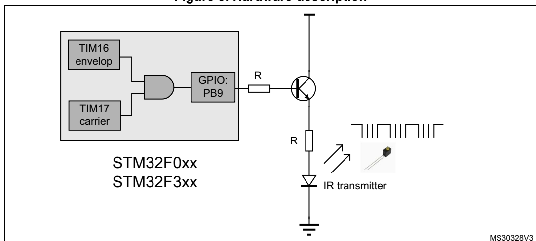
Figure 8. Hardware description
