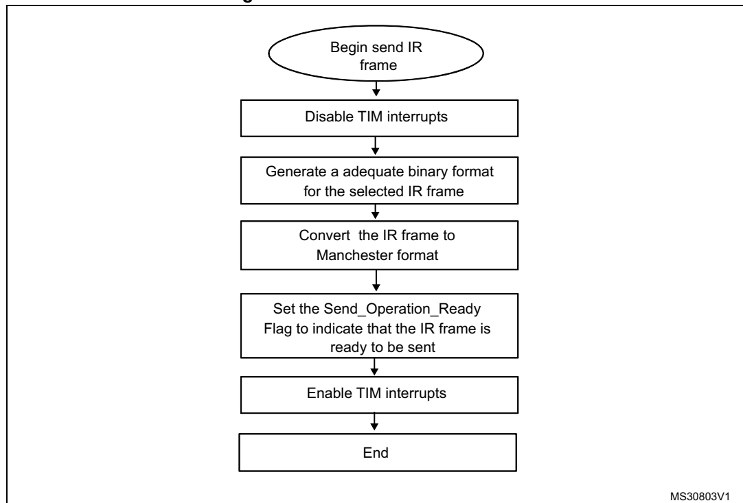
Figure 10. Send IR frame flowchart
