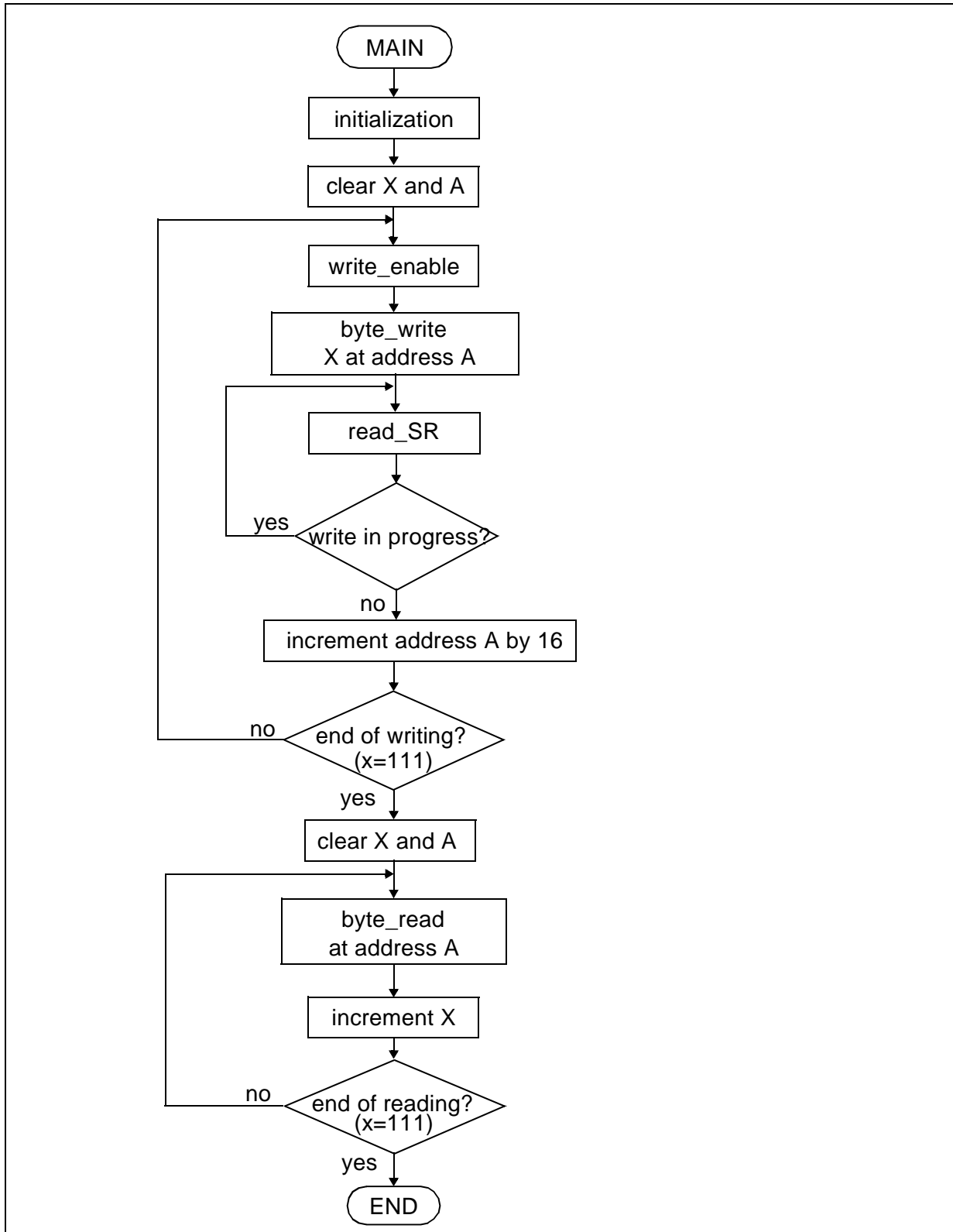
Figure 3. Flowchart: MAIN
