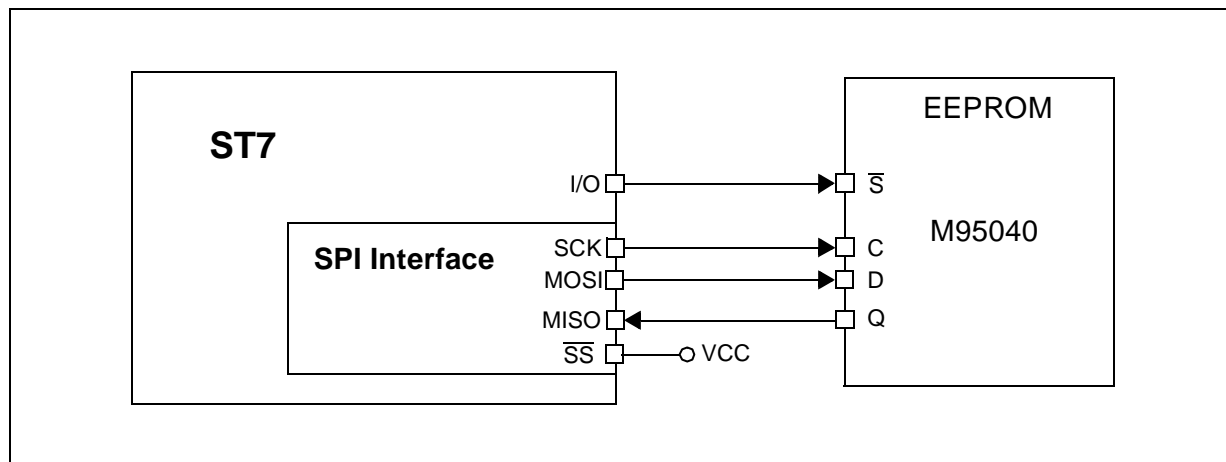
Figure 1. ST7 and SPI Interface Set-Up
