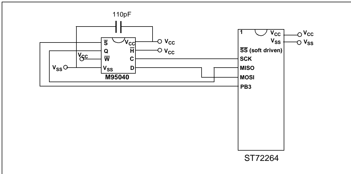
Figure 2. Hardware description
