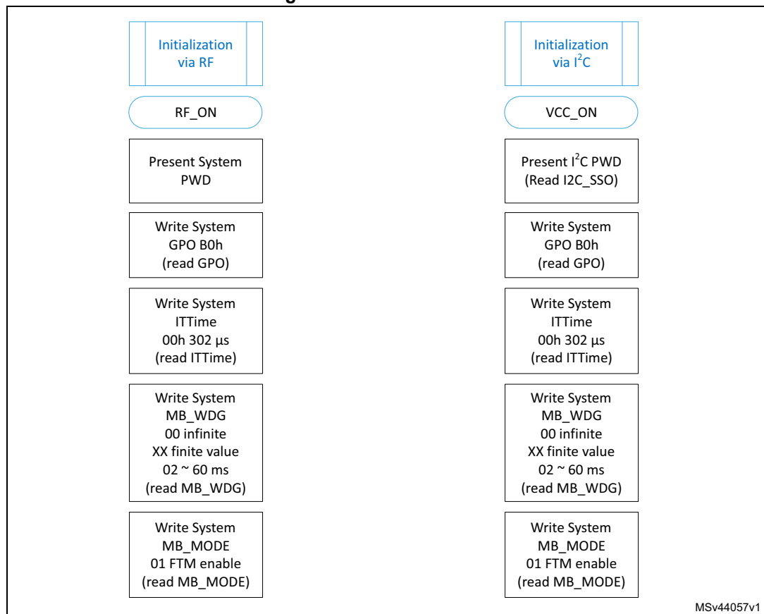
Figure 1. FTM initialization
