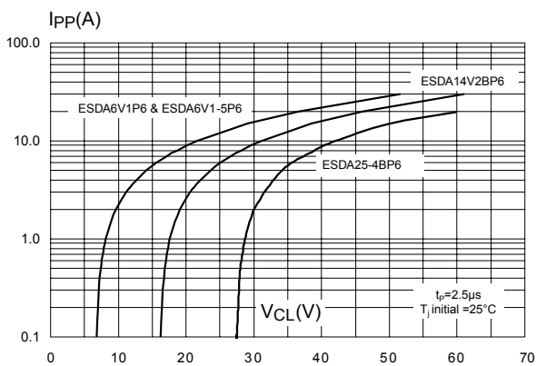
Figure 5. Clamping voltage versus peak pulse current ( T_j initial = 25° C, rectangular waveform, t_p = 2.5 \mu\text{s} )
